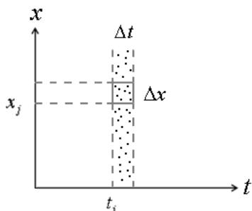
Fig.2 The description of random discontinuous motion of a single particle
