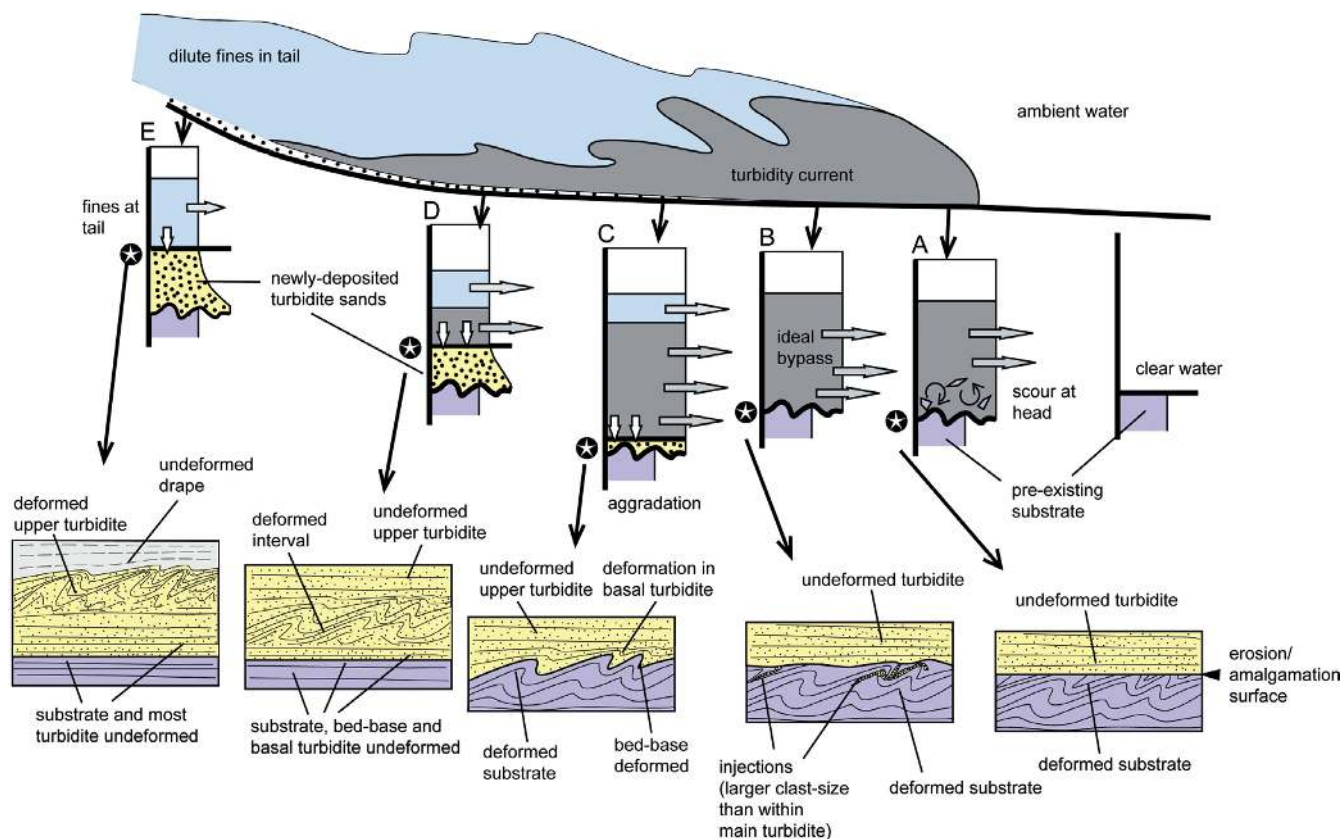
Fig. 9. Summary of locations and timing of deformation beneath an idealized turbidity current. If the head of the flow is erosive (A), any substrate deformation structures are prone to decapitation and sands deposited by subsequent parts of the flow will aggrade across these structures (e.g. Fig. 1g). Behind the head (B), but prior to significant deposition from the flow, deformation of the substrate can incorporate sediment from the turbidity current, siphoned into fractures and preserved as injections (e.g. Fig. 1c). Should deformation of the substrate happen as sediment is being deposited (C), the substrate, lower part of the overlying bed and their common interface will be deformed (e.g. Fig. 5). Deformation might begin after some sediment has been deposited from the turbidity current (D), creating strata-bound deformed intervals within the aggraded bed (e.g. Fig. 7). Finally, deformation might happen towards the rear of the turbidity current (E), represented by sheared bed-tops draped by siltstones (e.g. Fig. 1f). Some or all of these relationships between deformation and deposition can happen at the same site during the passage of a single turbidity current, creating tiered deformation through a turbidite sandstone and its immediate substrate.
