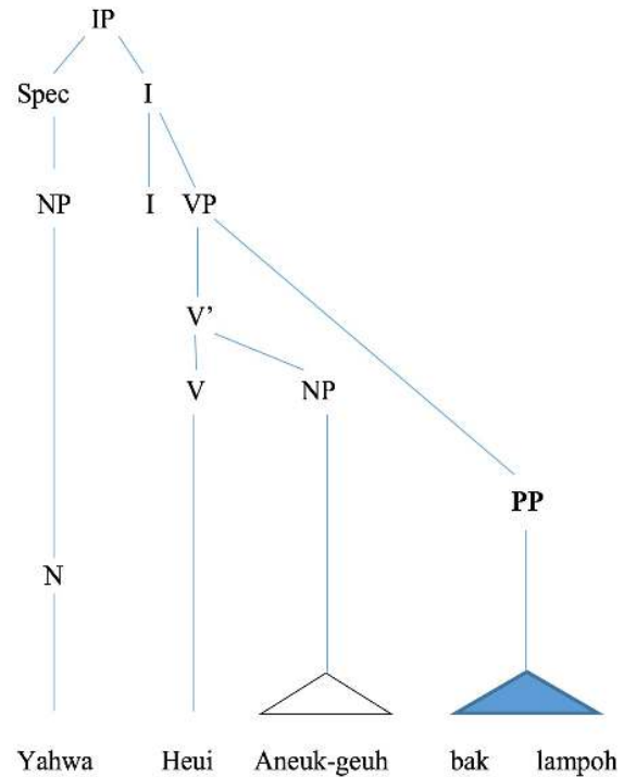
Fig.1. Declarative sentence
