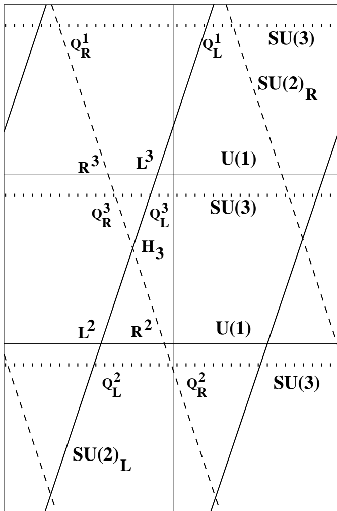
Figure 4: The SU(3) \times SU(2)_L \times SU(2)_R \times U(1) model of figure 2. Several torus fundamental domains are shown to highlight the relative size of the different Yukawa couplings. To avoid clutter, we do not show all the copies of the branes. Also, we only highlight the Yukawa couplings involving the Higgs field H_3 , hence do not show other fields living at the relevant intersections. World-sheets giving rise to quark (lepton) Yukawa couplings correspond to triangles with one vertex ( H_3 ) containing the Higgs and other two vertices Q_L^i, Q_R^i ( L^i, R^i ) containing the quarks (leptons).
