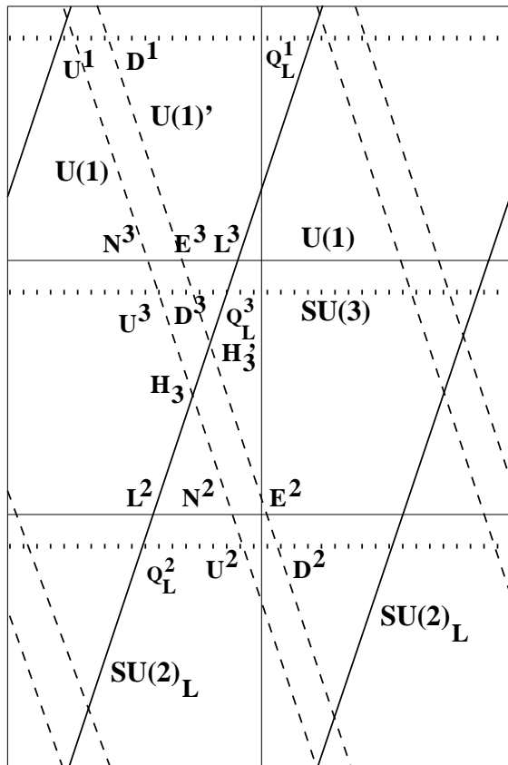
Figure 5: A standard model-like configuration obtained from that in figure 4 by splitting the SU(2)_R D4-branes into two parallel U(1) -branes. Now the size of the triangles corresponding to u- and d-quark Yukawa couplings are different.
