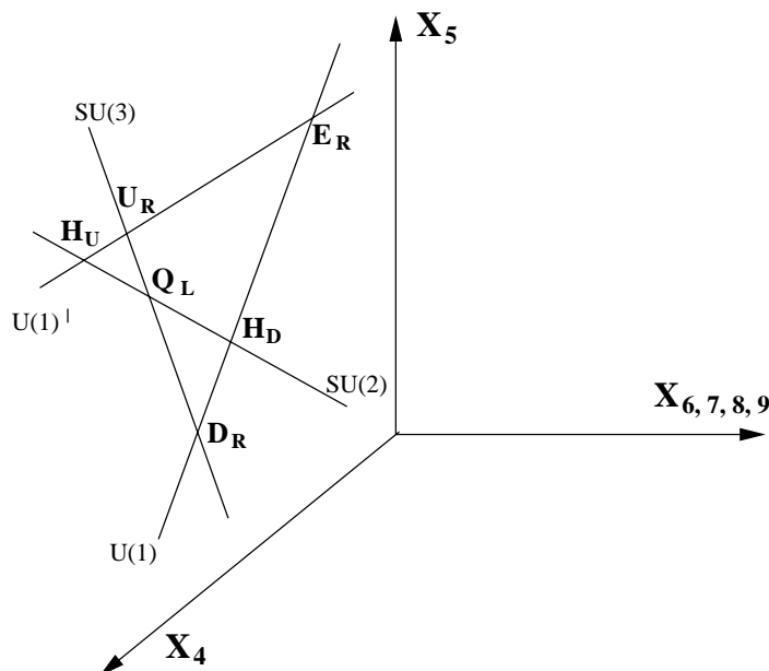
Figure 1: A simplified picture of the intersecting brane world scenario. Each gauge interaction propagates along a D-brane with four flat dimensions (not shown in the figure), and partially wrapped on a cycle in the internal space parameterized by X_4 , X_5 (a two-torus in our models). All branes are transverse to the space parameterized by X_6 , X_7 , X_8 , X_9 . Chiral fermions, such as quarks and leptons, are localized at the intersections of the wrapped branes (for simplicity, we have shown only one such intersection, even though generically multiple intersection points exist).
