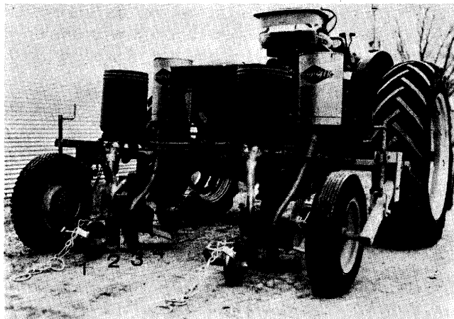
FIG. 1. The Bushland Range Interseeder showing (1) packer wheel, (2) seed placements, (3) fertilizer placements, (4) sweep, (5) coulter.
