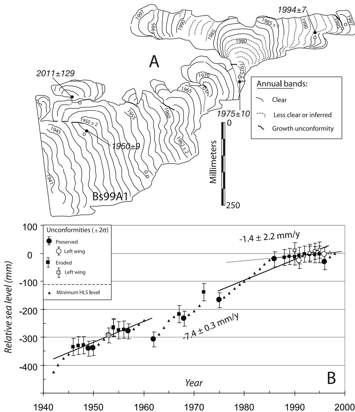
Figure 7. (a) Cross section of the modern Beusak slab and (b) graph of its HLS history. The low interior flat and high flat of the outer raised rim formed during periods of relative HLS stability. The thin arm that separates them grew during the period 1962–1985, when HLS unconformities were uncommon. The long-term average rate of submergence is about 7.4 \text{ mm yr}^{-1} , but the rate has been much slower since about 1985.
