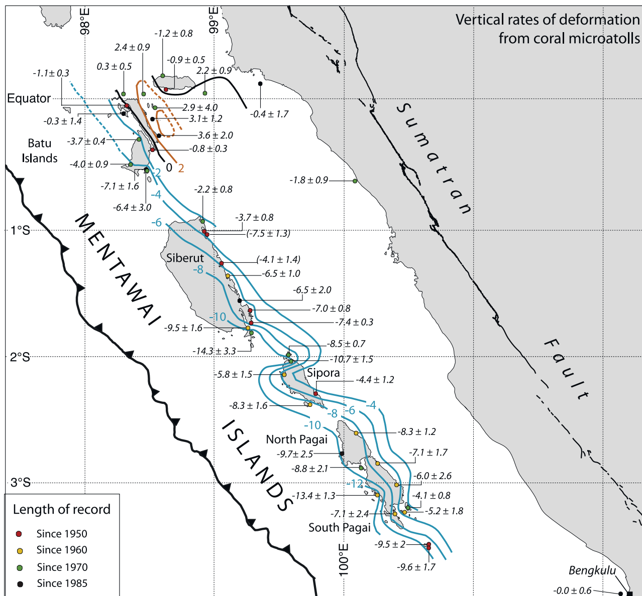
Figure 9. Map of average rates of subsidence of the Mentawai and Batu islands for the latter half of the 20th century. Contours show that, in general, rates increase southwestward toward the trench. Rates are anomalously high in the strait between Siberut and Sipora islands. The anomalously high value near 1°S is ignored in the contouring. Color coding of sites indicates the period spanned by the microatoll record. Uncertainties are 1\sigma .
