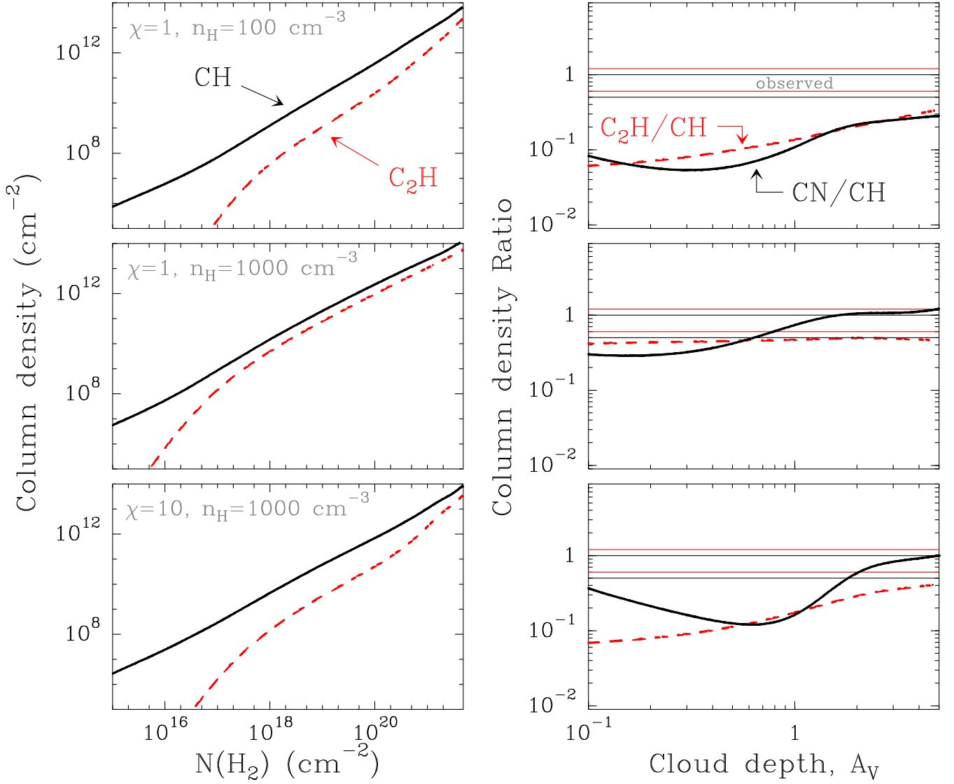
Fig. B.1. Left: Predicted variation of the CH (black line) and C 2 H (red dashed line) column density as a function of the H 2 column density for three models, computed with \zeta_H = 10^{-16} \text{ s}^{-1} : \chi=1 and n_H = 100 \text{ cm}^{-3} (top), \chi=1 and n_H = 1000 \text{ cm}^{-3} (middle) and \chi=10 and n_H = 1000 \text{ cm}^{-3} (bottom). Right: Variation of the CN/CH (black lines) and C 2 H/CH (red dashed lines) column density ratios for the same models. The gas density n_H is defined as n(H) + 2n(H_2) . The observed ranges are indicated.
