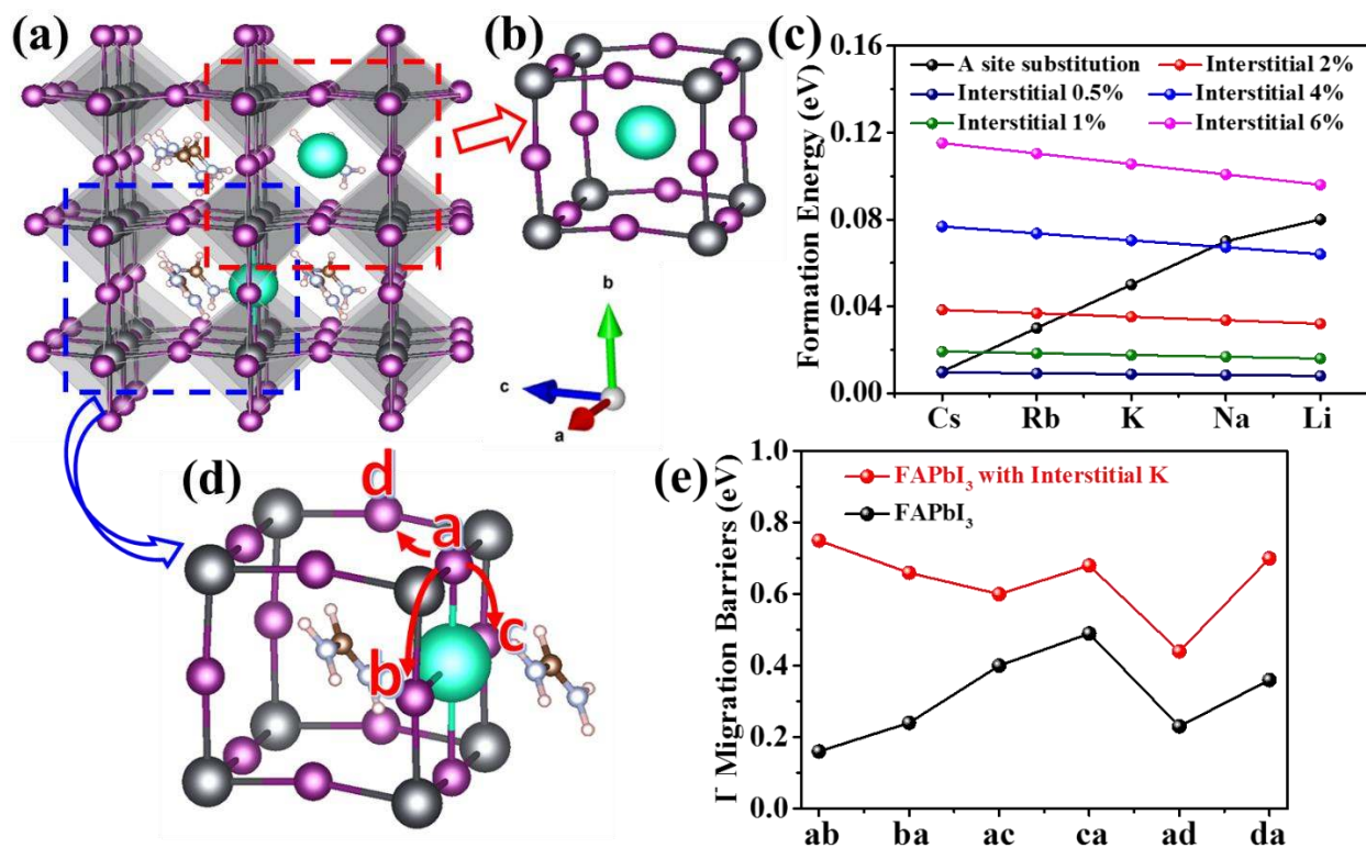
Figure 2. Thermodynamic and kinetic properties of alkali cation incorporation ( \text{Cs}^+ , \text{Rb}^+ , \text{K}^+ , \text{Na}^+ , and \text{Li}^+ ). (a) Illustration of the possible locations of alkali cations in \text{FAPbI}_3 : (b) at the A site and (d) at the interstitial site. (c) \Delta H_{0\text{K}} of alkali cation incorporation at an A site (being constant for concentration from 0.5% to 6%) and at an interstitial site. Values are estimated based on Table S2 and Figure S3. (d) Illustration of the \text{I}^- diffusion pathways, using \text{FAPbI}_3 perovskite with \text{K}^+ at an interstitial site as an example. (e) Comparison of the \text{I}^- diffusion barriers in \text{FAPbI}_3 with and without interstitial \text{K}^+ . The lines are guides to the eye.
