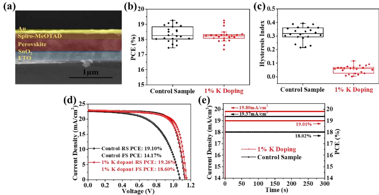
Figure 4. Impact of interstitial doping on PSC performance. (a) Cross-sectional SEM image of the PSC structure. (b) Comparison of the PCE (extracted from the reverse scans of the J-V curves) of the PSCs without doping and with 1% \text{K}^+ doping. (c) Comparison of the hysteresis index of the PSCs without doping and with 1% \text{K}^+ doping. The statistics of the PCE and hysteresis index in (b) and (c) are based on 22 devices for each condition. The tiny box within the large box indicates mean value. The upper and lower bars represent standard deviation from the mean value, and the middle line in each box represents the median value. Upper and lower borderlines of the box represent the third quartile (Q3) and first quartile (Q1), respectively, and box thickness represents interquartile range \text{Q3-Q1} . (d) J-V curves from the reverse and forward scans of the PSCs without doping and with 1% \text{K}^+ doping. (e) Steady-state current density and PCE of the PSCs without
