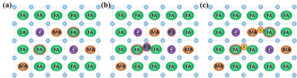
Figure 3. Schematics of the doping mechanism of Cs/MA/FA perovskite doped with Cs + , Rb + , and K + . (a) Side view of the original Cs/MA/FA perovskite lattice structure. (b) Side view of the lattice structure of Cs/MA/FA perovskite doped with Rb + . (c) Side view of the lattice structure of Cs/MA/FA perovskite doped with K + .
