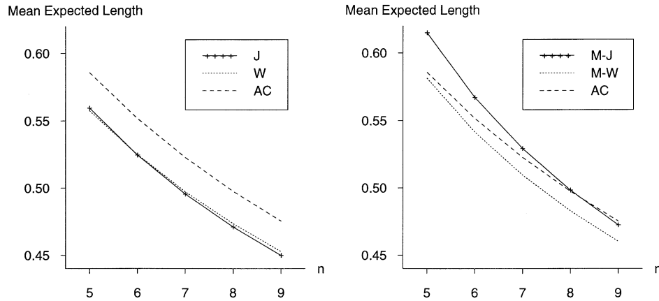
FIG. 1. A Comparison of mean expected lengths for the nominal 95% Jeffreys ( J ), Wilson ( W ), Modified Jeffreys ( M\text{-}J ), Modified Wilson ( M\text{-}W ), and Agresti–Coull ( AC ) intervals for n = 5, 6, 7, 8, 9 .
