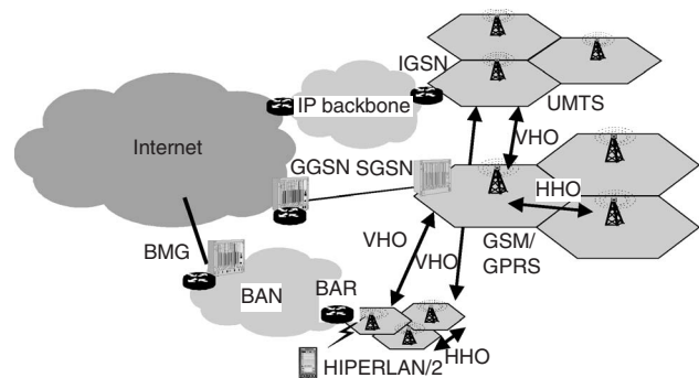
Fig. 1 Horizontal and vertical handover in MIND
