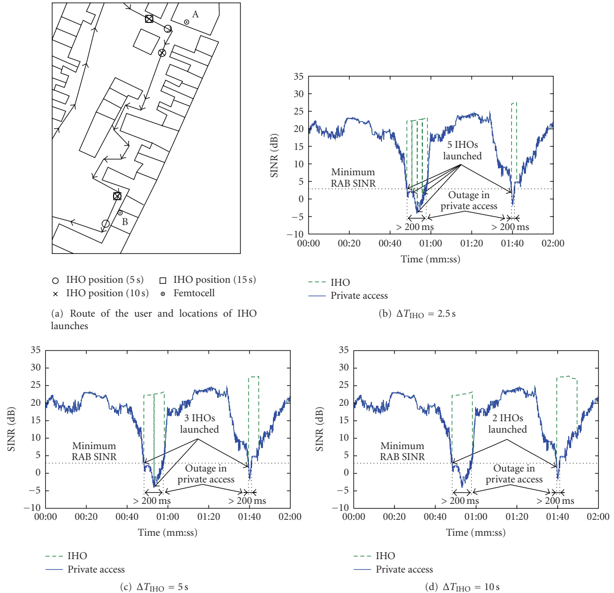
FIGURE 4: Performance comparison of CSG and IHO for a mobile nonsubscriber ( \Delta Q_{IHO} = 3 dB).
