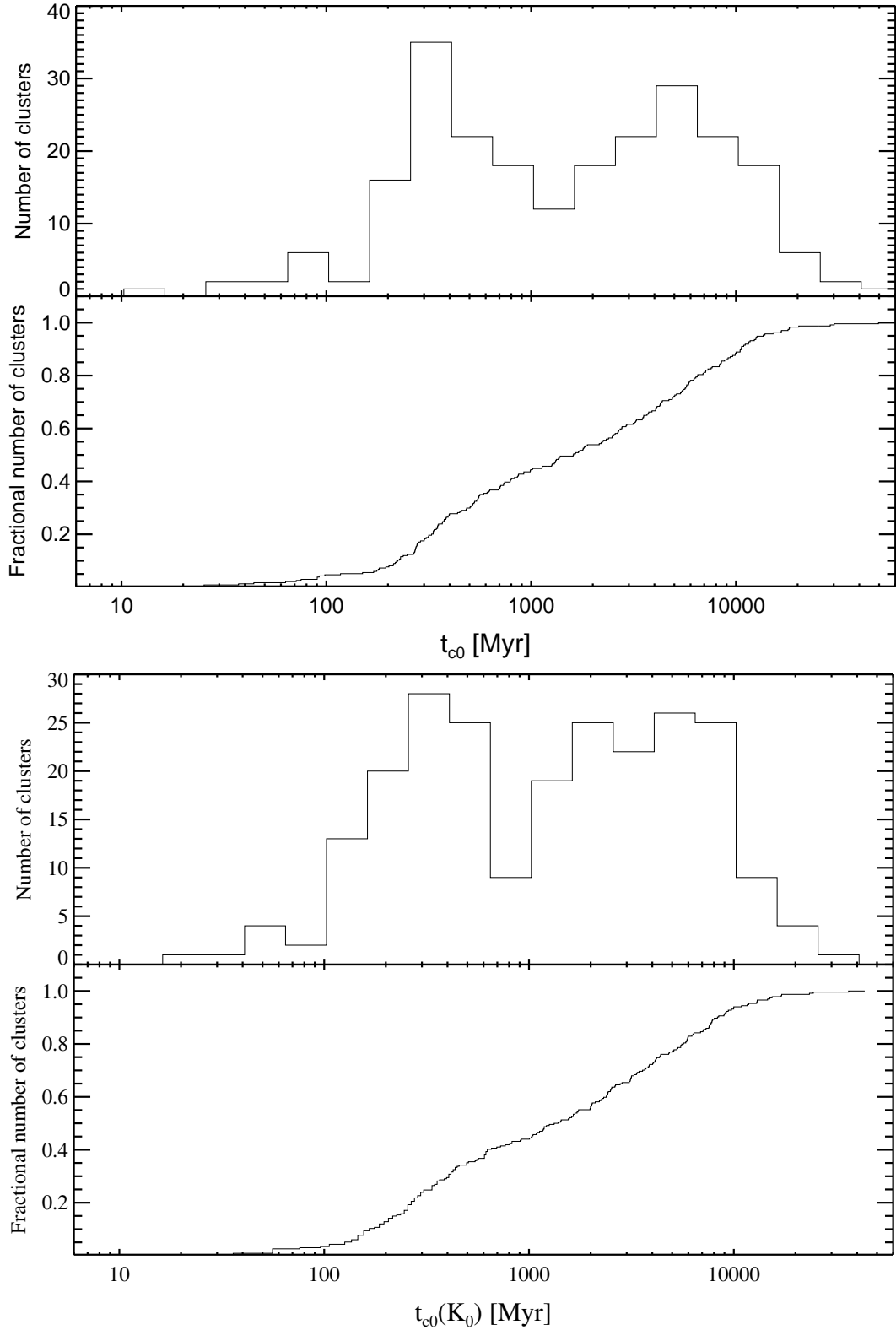
FIG. 8.— Top panel : Log-binned histogram and cumulative distribution of best-fit core cooling times, t_{c0} (eqn. 8), for all the clusters in ACCEPT . Histogram bin widths are 0.2 in log space. Bottom panel : Log-binned histogram and cumulative distribution of core cooling times calculated from best-fit K_0 values, t_{c0}(K_0) (eqn. 9), for all the clusters in ACCEPT . Histogram bin widths are 0.2 in log space. The bimodality we observe in the K_0 distribution is also present in best-fit t_{c0} . However, the gaps between the two populations of t_{c0} and t_{c0}(K_0) differ by \sim 0.3 Gyr which may be an artifact of the binning.
