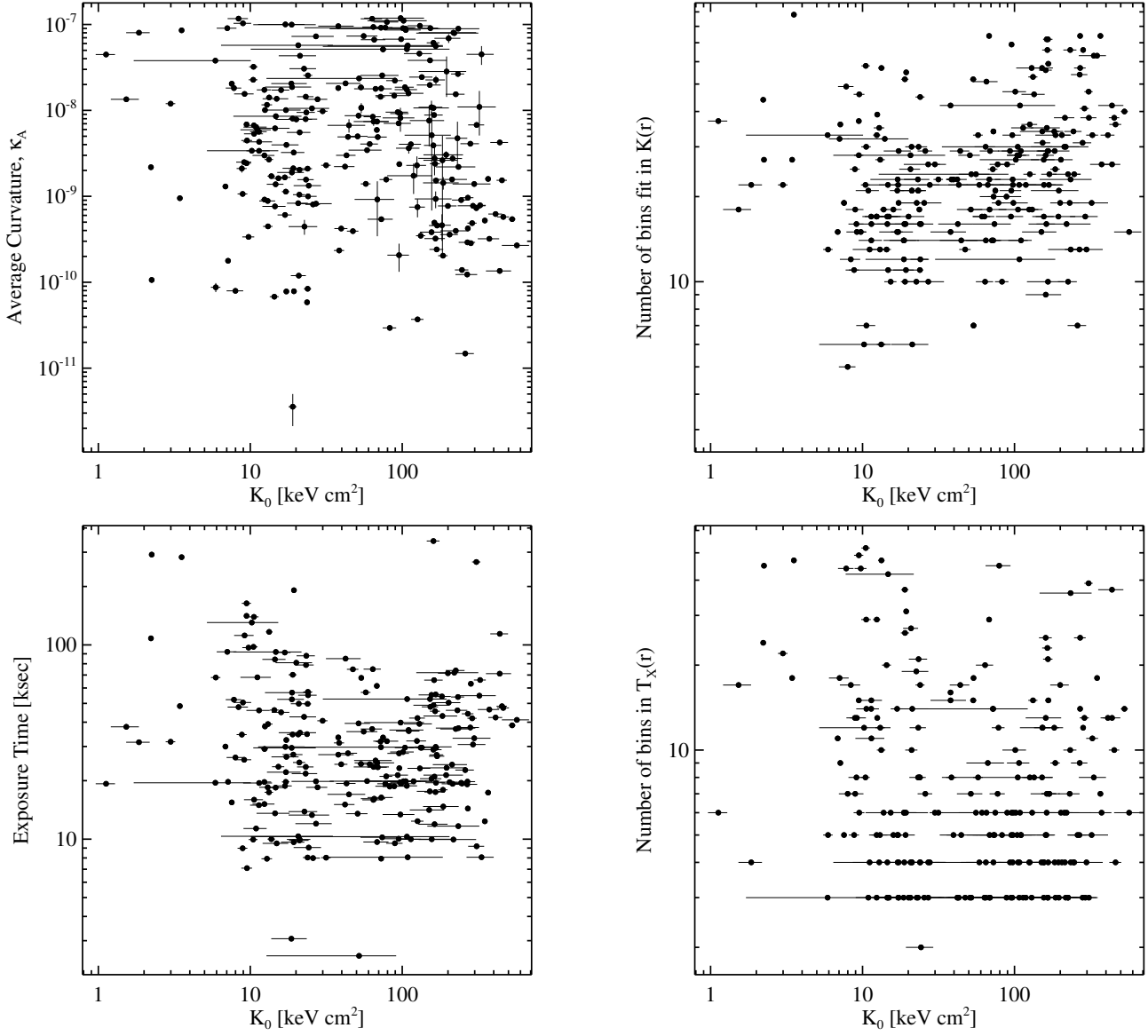
FIG. 4.— Plots of possible systematics versus best-fit K_0 . Top left : Best-fit K_0 plotted versus average curvature of the corresponding entropy profile (see eq. 6). There is no trend between these two quantities suggesting that K_0 is not heavily influenced by the total shape of the entropy profile. Top right : Best-fit K_0 plotted versus number of bins in the entropy profile which were used during fitting. Again, no trend is found. Bottom left : Best-fit K_0 plotted versus the total used exposure time for each cluster. No trend is found. Bottom right : Best-fit K_0 plotted versus the number of bins in the temperature profile for each cluster. As expected, fewer T_X(r) does not correlate with K_0 .
