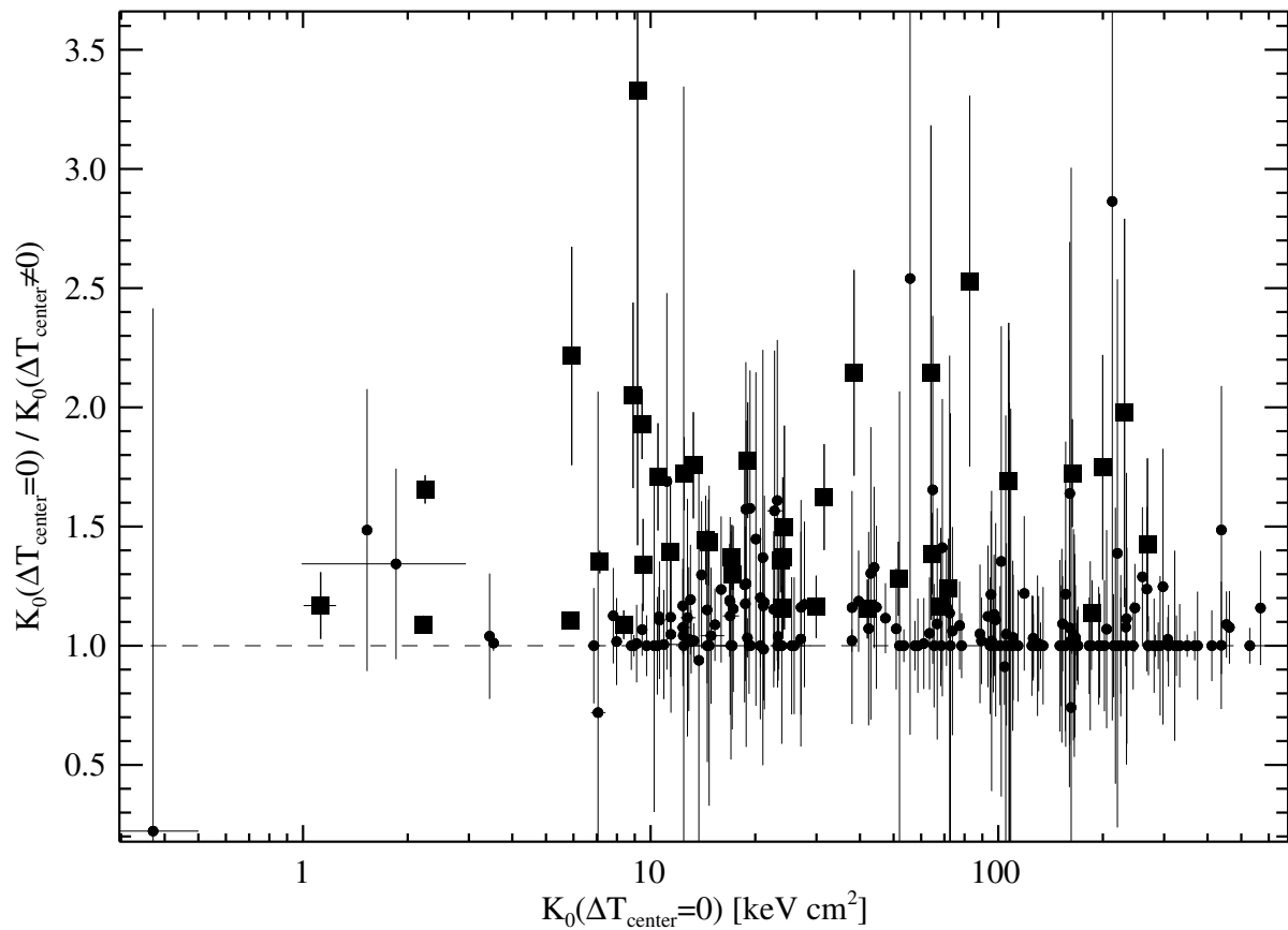
FIG. 2.— Ratio of best-fit K_0 for the two treatments of central temperature interpolation (see §3.1): (1) temperature is free to decline across the central density bins ( \Delta T_{center} \neq 0 ), and (2) the temperature across the central density bins is isothermal ( \Delta T_{center} = 0 ). Filled black squares are clusters for which the K_0 ratio is inconsistent with unity.
