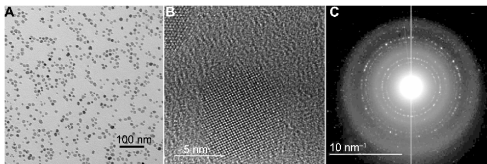
Figure 1 Transmission electron microscopy images of the magnetic nanoparticles. (A) Particle cores measured to be 11.3 ± 2.3 nm (scale bar = 100 nm). (B) High-resolution lattice image of a 9.9 nm particle showing its crystalline core (scale bar = 5 nm). (C) Electron diffraction pattern, identifying cores as Fe 3 O 4 (scale bar = 10 nm -1 ).
