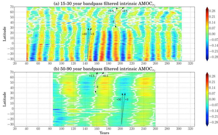
FIG. 10. Time–latitude plots of intrinsic AMOC_{\sigma_2} anomalies ( Sv ) during the 1/4^\circ S run, bandpass filtered (top) in the 15–30-yr band and (bottom) in the 50–90-yr band; initial and final parts of the time series are ignored because of the side effects of the Lanczos filters. Slanted lines and associated numbers indicate ranges of meridional phase speeds ( cm\ s^{-1} ) that dominate within selected latitude ranges; pluses and minuses correspond to northward and southward propagation, respectively.
