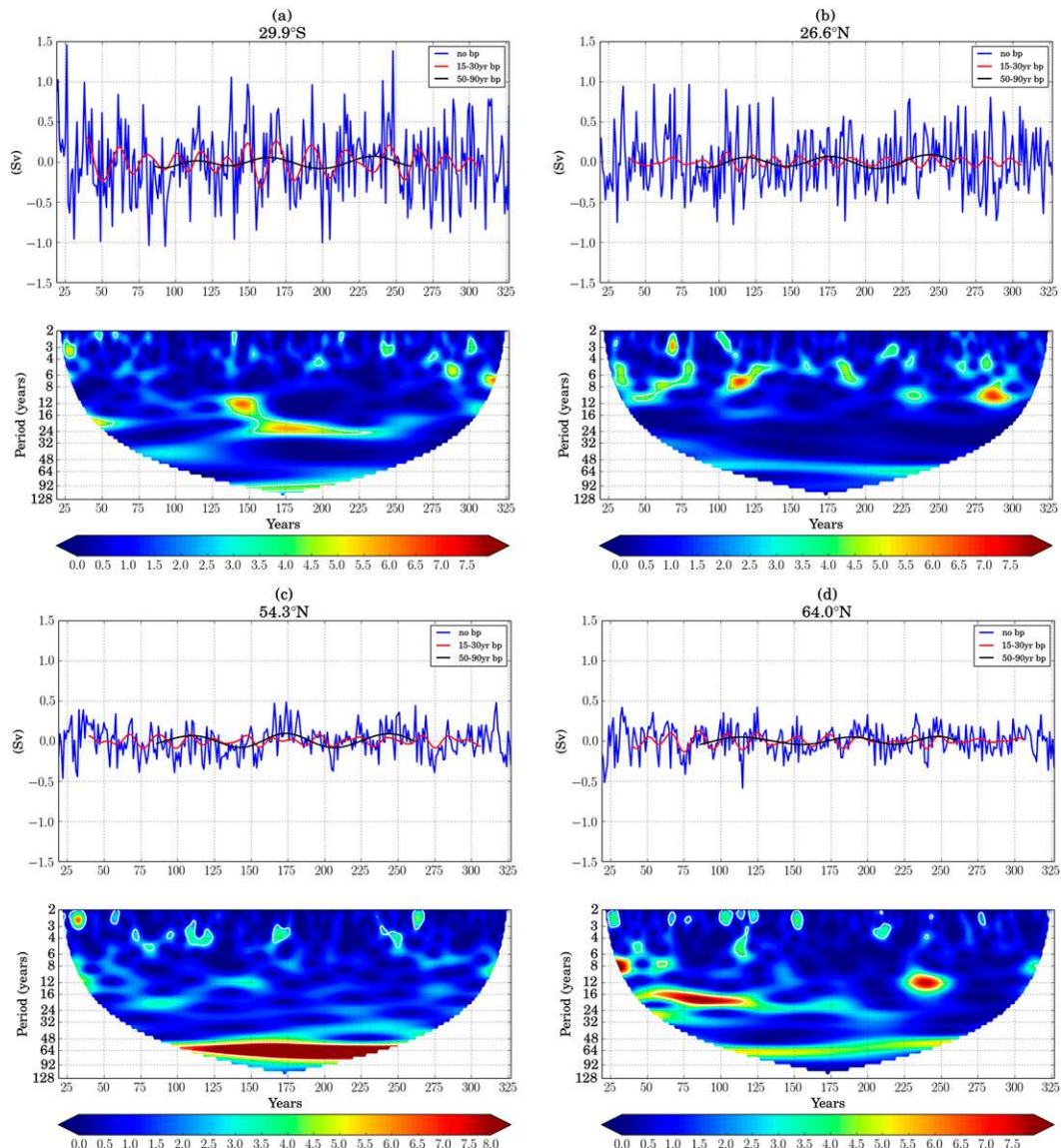
FIG. 8. Intrinsic AMOC_{\sigma_2} anomaly time series and wavelet power spectra from the last 309 yr of the \frac{1}{4}^\circ S run at (a) 29.9^\circ S, (b) 26.6^\circ N, (c) 54.3^\circ N, and (d) 64^\circ N. Shown are unfiltered (blue) and bandpass-filtered yearly time series in the 15–30- (red) and 50–90-yr (black) bands, for comparison with Fig. 10. Wavelet spectra are normalized by the variance of time series; white contours indicate 95% confidence levels.
