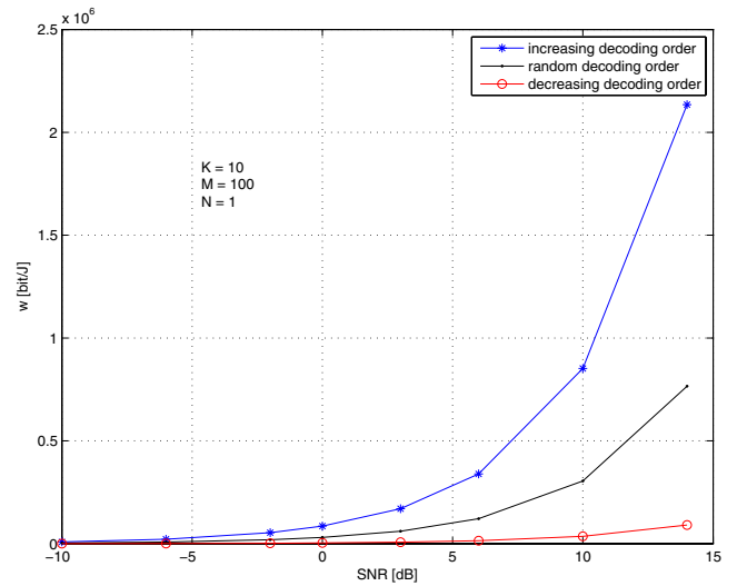
Fig. 1. Influence of the decoding order on the social welfare.
