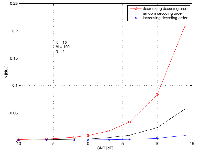
Fig. 2. Influence of the decoding order on the equivalent virtual MIMO network energy efficiency.
