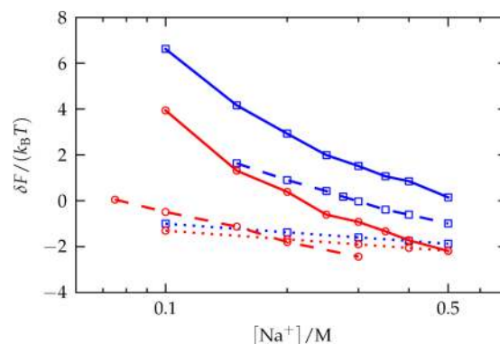
FIG. 12. The free energy difference between the bound and unbound state for two hairpins as measured in experiment using FRET (dashed lines), and as predicted by oxDNA2 (solid lines) and the SantaLucia model (dotted lines). Results for two different hairpins are presented: the A_{31}\text{-VW} (red, circular markers) hairpin and the T_{31}\text{-VW} hairpin (blue, square markers). The sequences for these hairpins are given in Table S4. 69 The oxDNA2 simulations were run for 10^{10} VMMC steps for each hairpin, with q_{\text{eff}} = 0 and x = 0 (with x defined in Eq. (10)), and the results (computed for the standard oxDNA2 values for q_{\text{eff}} and x ) were calculated using thermodynamic integration as described in Sec. VI and Sec. II C of the supplementary material. 69
