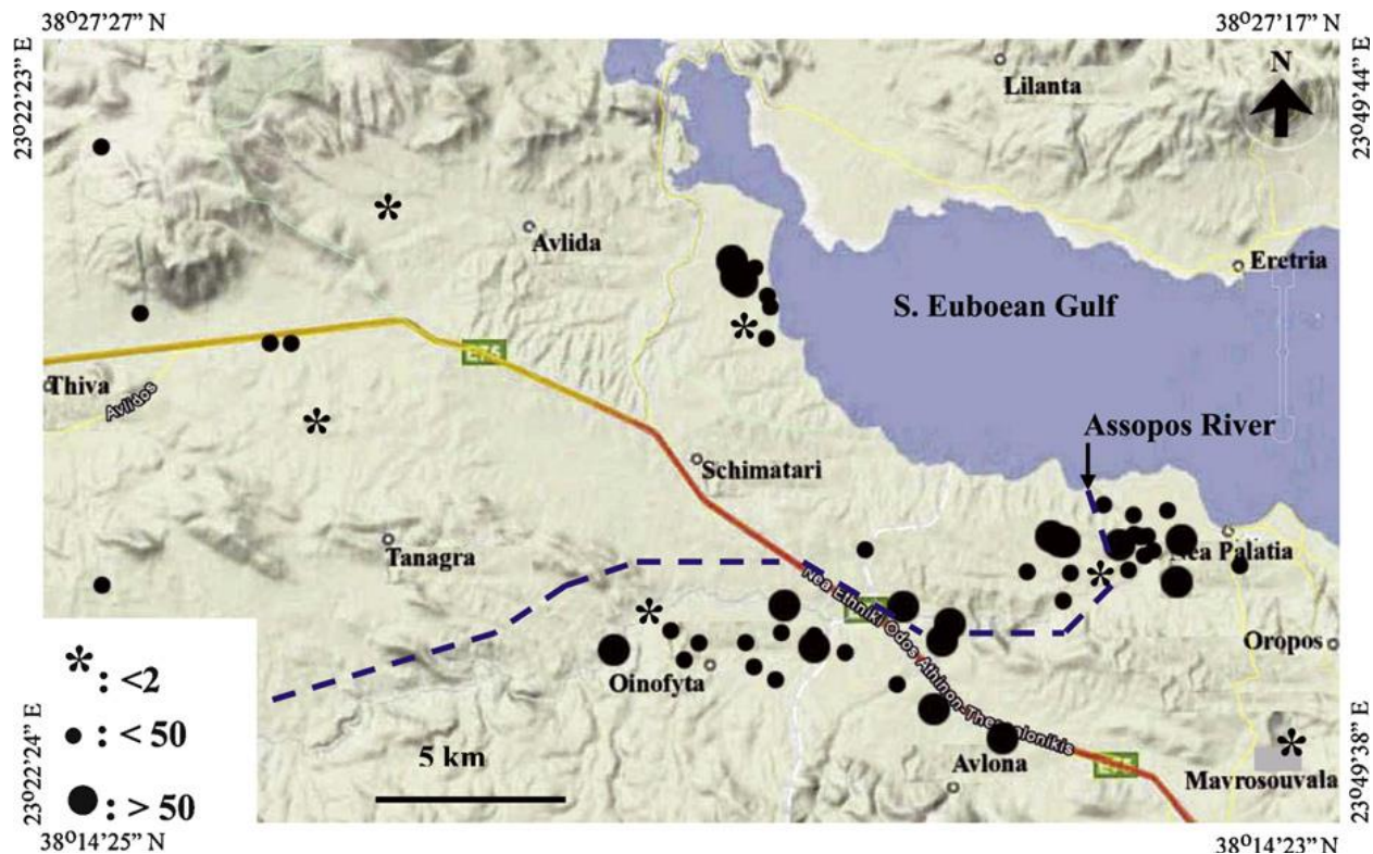
Figure 3: Location of the groundwater boreholes and distribution of the Cr_{total} concentration (in ppb) throughout the Asopos basin. The groundwater samples were classified into three groups: (a) lower than 2 ppb Cr_{total} , (b) lower than 50 ppb Cr_{total} , and (c) higher than 50 ppb Cr_{total} . Source: Economou-Eliopoulos et al. (2011, p.45)
