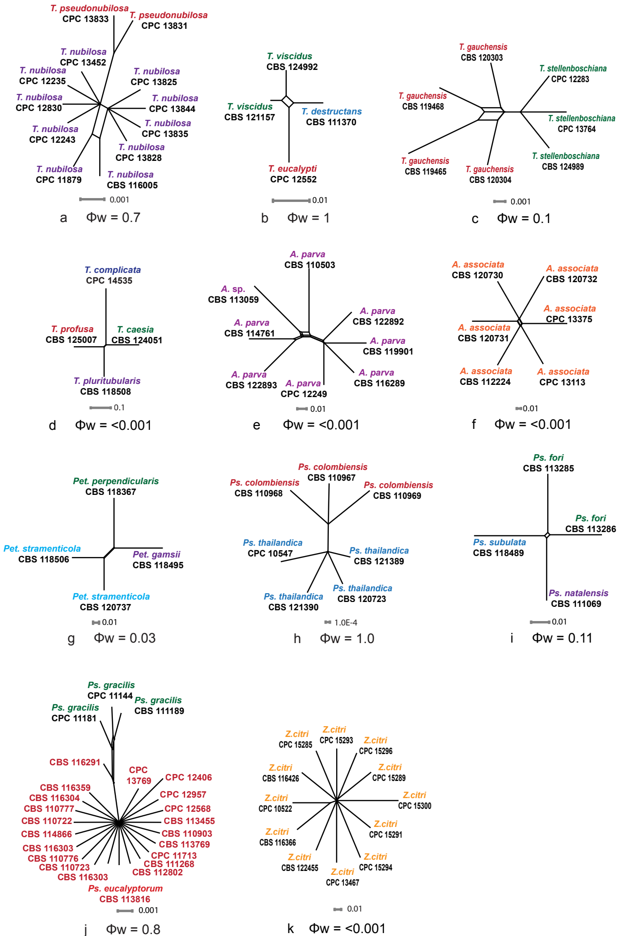
Fig. 6 The results of the pairwise homoplasy index (PHI) test of closely related species using both LogDet transformation and splits decomposition. PHI test results ( \Phi_w < 0.05 ) indicate significant recombination within the dataset.
