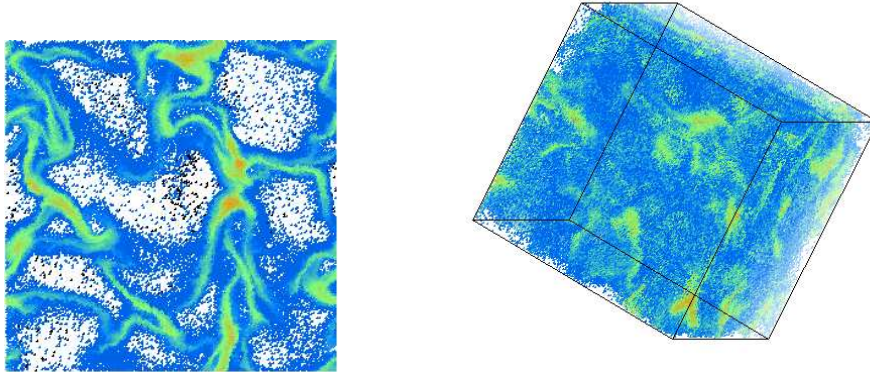
Figure 12. (Left) Collision frequency of individual particles from a 2D simulation, after about 5200 collisions per particle. (Right) Cluster visualization from a 3D simulation. The colors in both panels indicate large (red), medium (green), and small (blue) collision rates.
