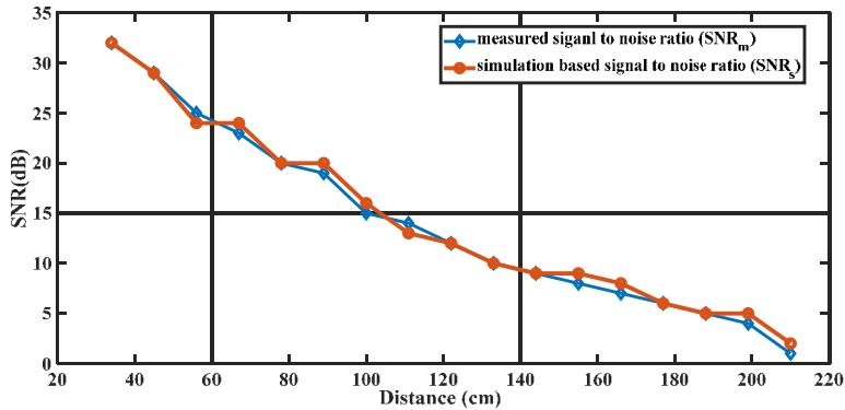
Figure 9: Simulation-based and measured SNR under varying distance under a LiFi attocell.
