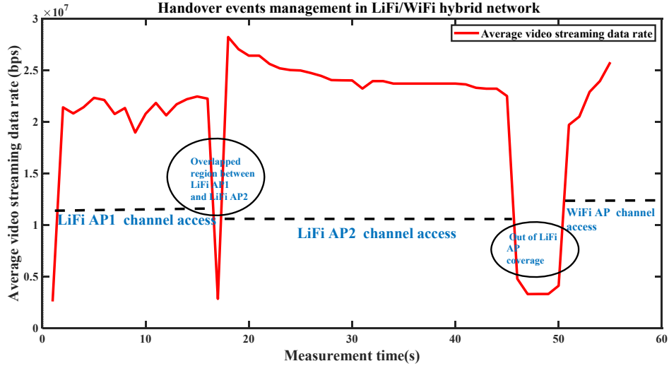
Figure 8: Measured average data rate during handover of user device from LiFi to LiFi and LiFi to WiFi.
