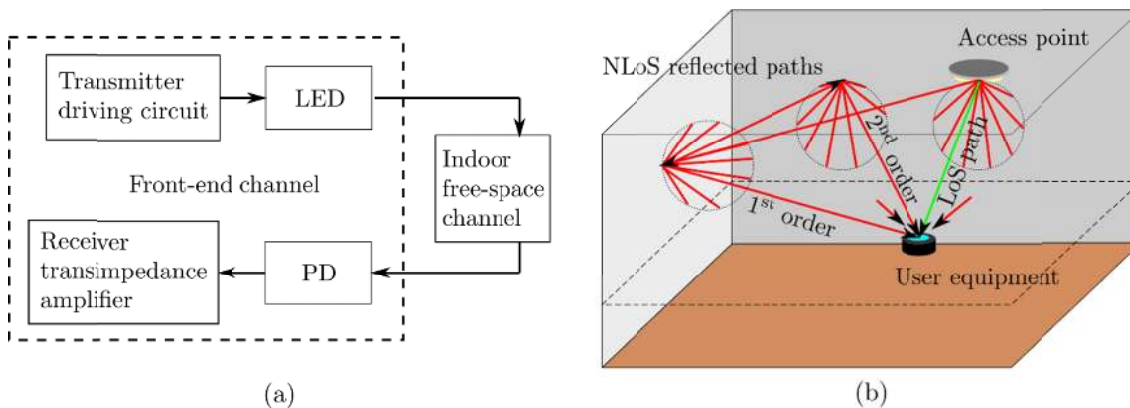
Figure 2: (a) LiFi channel block diagram. (b) Illustration of indoor free space VLC channel.
