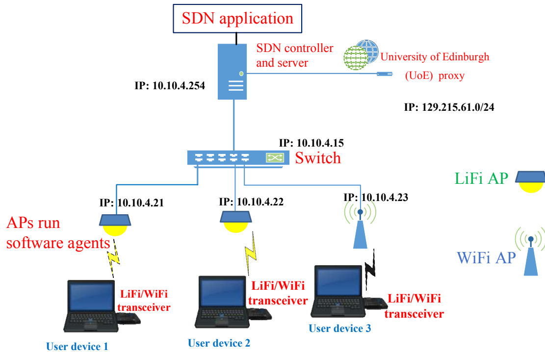
Figure 7: Experimental SDN-enabled LiFi/WiFi network testbed diagram, LiFi R&D Centre, UoE
