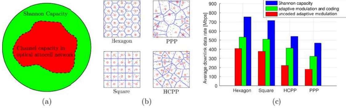
Figure 5: (a) Relationship between Shannon capacity upper bound and channel capacity in a LiFi network; (b) various cell layouts in LiFi networks. (c) Example of downlink performance in a LiFi network with an average cell radius of 2.5 m, a source half-power semiangle of 40°.
