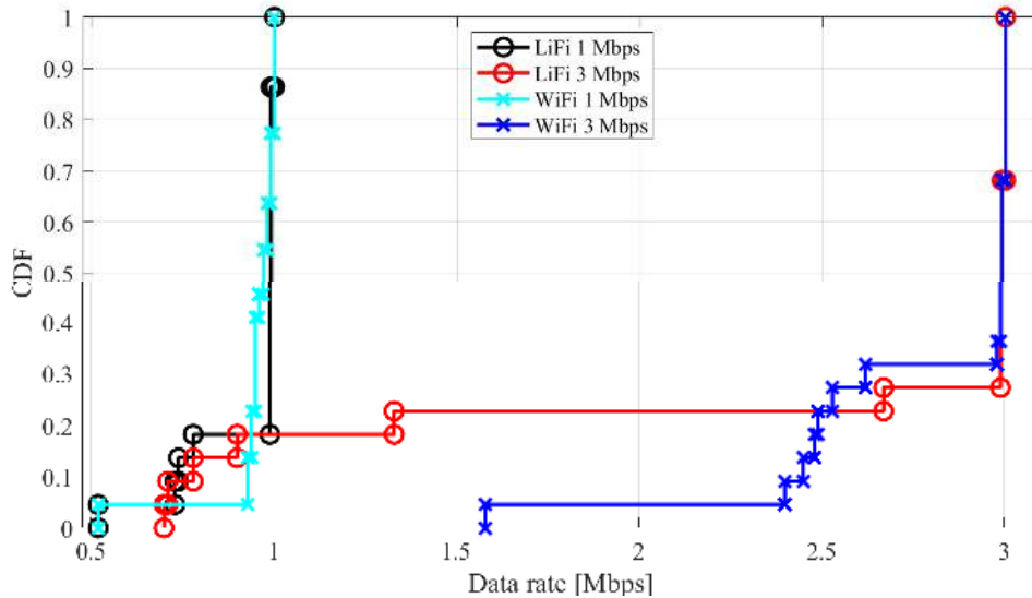
Figure 11: The CDF of the data rate for the Wi-Fi and LiFi users based on the 1 Mbps and 3 Mbps data rates targets.
