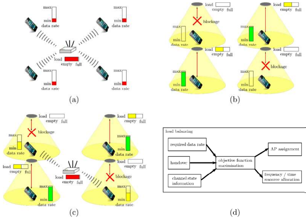
Figure 6: (a) Wi-Fi standalone network. (b) LiFi standalone network. (c) LiFi / Wi-Fi hybrid network. (d) Load balancing in LiFi / Wi-Fi hybrid network.
