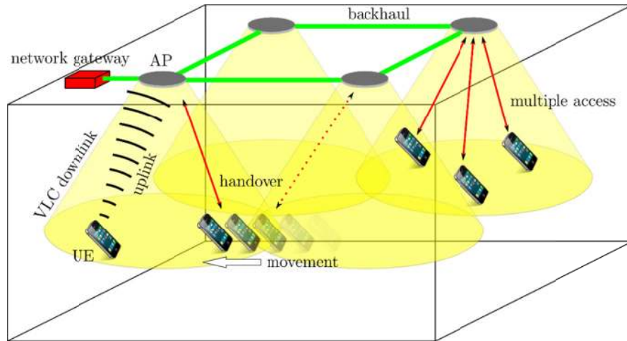
Figure 3: LiFi network illustration. A complete LiFi network includes downlink, uplink, and backhaul connections. In addition, the system should provide handover function, mobility support and multiple access capability.
