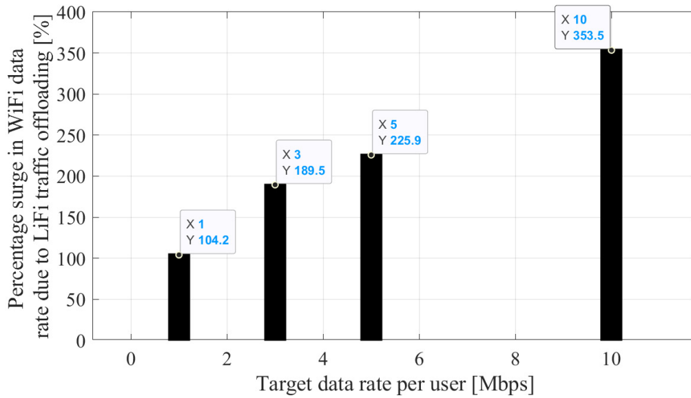
Figure 13: Surge in Wi-Fi aggregated data rate at neighbouring classrooms
