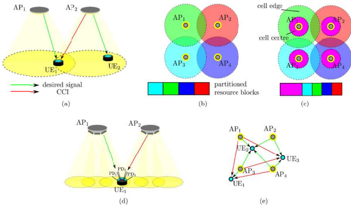
Figure 4: (a) Demonstration of co-channel interference (CCI). (b) Static resource partitioning (c) Fractional frequency reuse. (d) Interference coordination with angular diversity transmitters and receivers. (e) Cooperative multi-point joint transmission.
