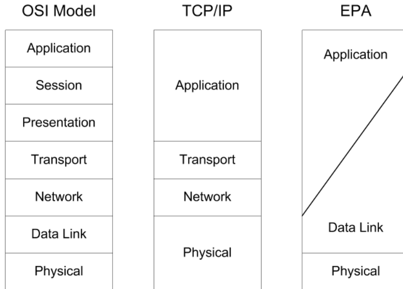
Fig. 3. Comparison of network stack configurations
