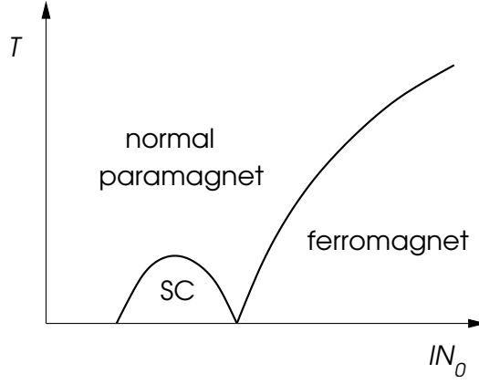
FIGURE 6. Schematic phase diagram of the superconducting phase (SC) near the ferromagnetic quantum critical point.
