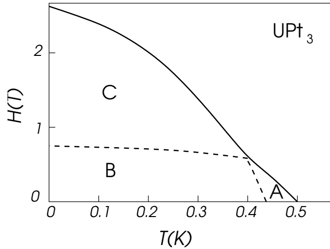
FIGURE 13. Phase diagram of \text{UPt}_3 : There are two consecutive superconducting transitions in zero magnetic field, distinguishing the phase A and B [49]. The phase B is likely time reversal symmetry breaking [48]. In a magnetic field a third phase C is observed [50, 47].
