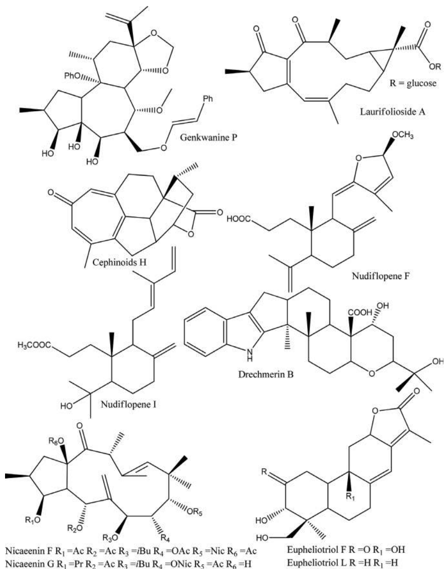
Figure 4. Structure of diterpenes.
