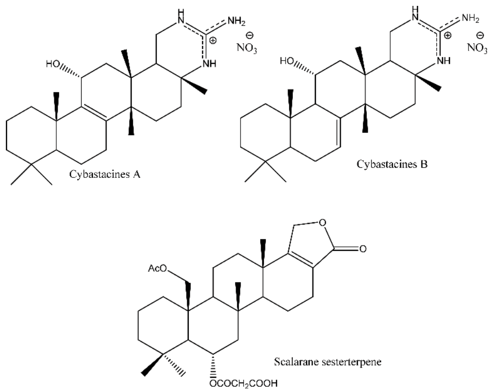
Figure 5. Structures of sesterpenes.
