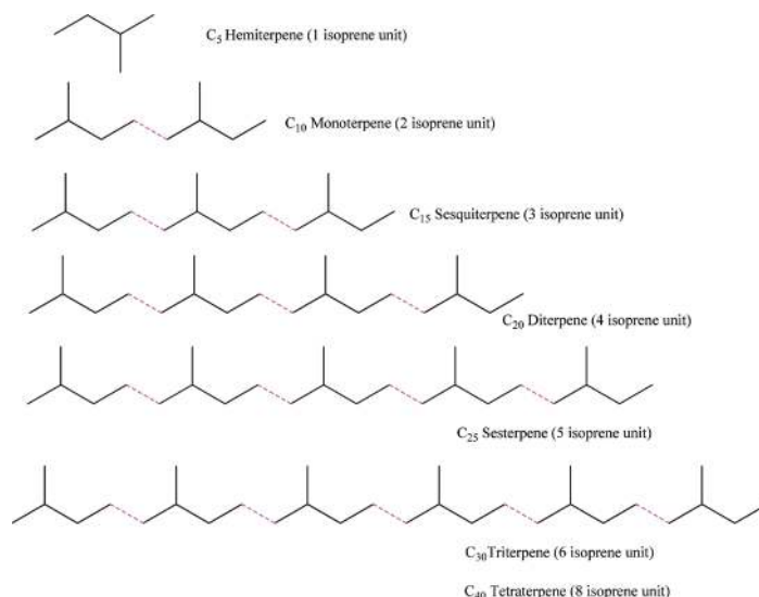
Figure 1. Classification of terpenes.
