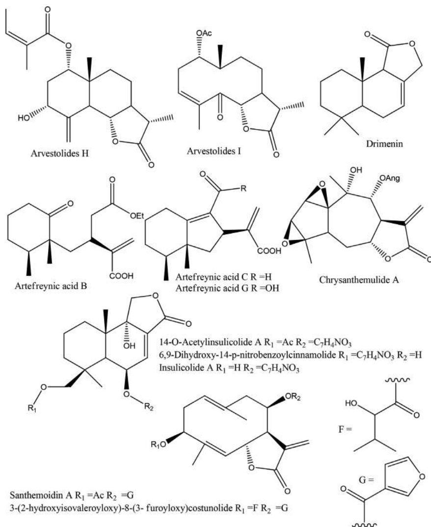
Figure 3. Structures of sesquiterpenes.
