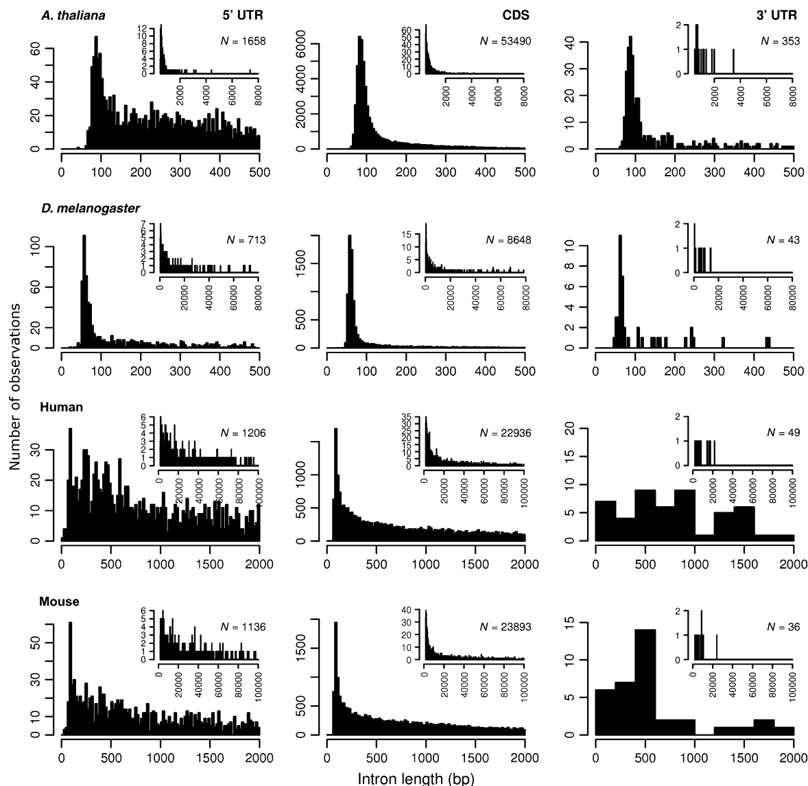
FIG. 1.—Intron length distributions in the 5' UTR (left), CDS (center), and 3' UTR (right) of full-length cDNA transcripts for Arabidopsis thaliana , Drosophila melanogaster , human, and mouse. The inset histogram continues the right tail of the main histogram with the identical bin size, so that the ordinate axes of the two histograms are on the same frequency scale. Bin sizes are 5 bp for A. thaliana and D. melanogaster and 20 bp for human and mouse, except for human and mouse 3' UTRs for which bin sizes are 200 bp due to small sample sizes.
