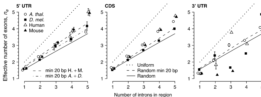
FIG. 4.—Intron dispersion within UTRs. Mean effective number of exons n_e \pm SE for regions containing 1–5 introns in the UTRs and the CDS. Lines indicate expected values of n_e for intron distributions having uniform exon sizes (dotted), random exons of minimum size 20 bp (dashed), and random exons of minimum size 1 bp (solid). For the 5' UTR, separate minimum 20 bp distributions are provided for human and mouse as a group (dashed) and Arabidopsis thaliana and Drosophila melanogaster as a group (dash-dot). Values above a random distribution indicate an overdispersed (more uniform) distribution, whereas those below a random distribution indicate an underdispersed (more clumped) distribution. See figure 3 for sample sizes; error bars are omitted where sample size < 5 . Error bars that are not visible when sample size \geq 5 are more narrow than the height of the plotting symbols.
