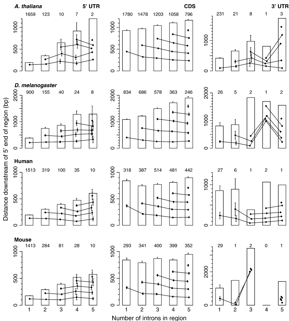
FIG. 3.—Mean intron positions within regions. Bars indicate mean length \pm SE of regions containing that many introns. Mean intron position \pm SE is plotted within each transcript bar so that its relative position within the mean region is apparent. Bars are oriented so that the 5' end of each region starts at 0. Introns occupying the same ordinal position within each region (first, second, etc.) are connected by lines across transcripts. The ordinate is identical for the 5' UTR and CDS of each species, and varies for the 3' UTR. Numbers above bars indicate sample sizes; error bars are omitted where sample size < 5 . Error bars that are not visible when sample size \geq 5 are more narrow than the height of the plotting symbols.
