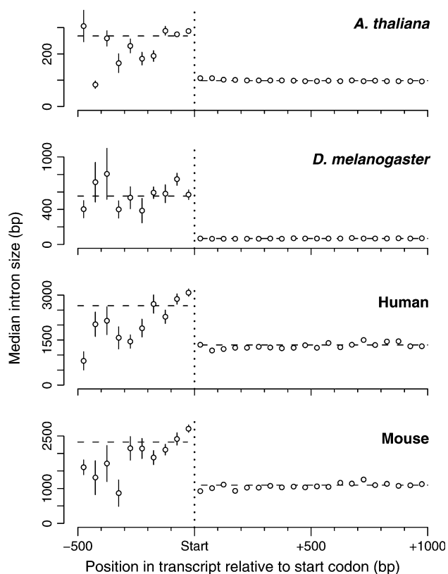
FIG. 2.—Median intron size versus relative position within transcript for all introns. For each species, the region to the left of the vertical dotted line is the 5' UTR, the region to the right is the CDS. Median intron sizes within each 5' UTR and CDS are indicated by horizontal dashed lines. Bin sizes are 50 bp. The total length of each error bar is equal to the interquartile distance divided by the square root of the sample size within each bin; note that some error bars are more narrow than the height of the plotting symbols.
