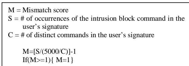
Figure 8: Mismatch score calculation
