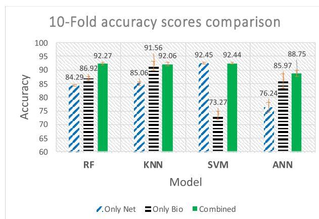
FIGURE 6. 10-Fold accuracy scores comparison.
