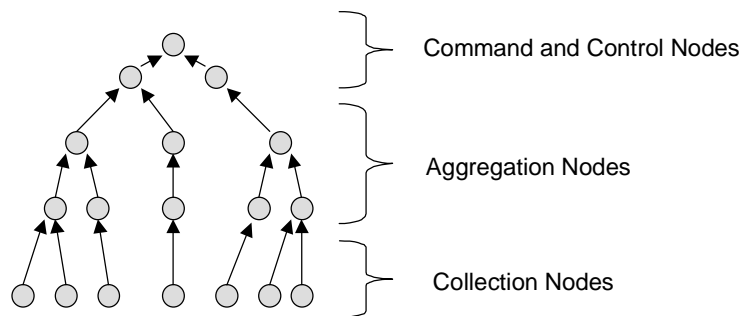
Figure 1: Hierarchical IDS Architecture
