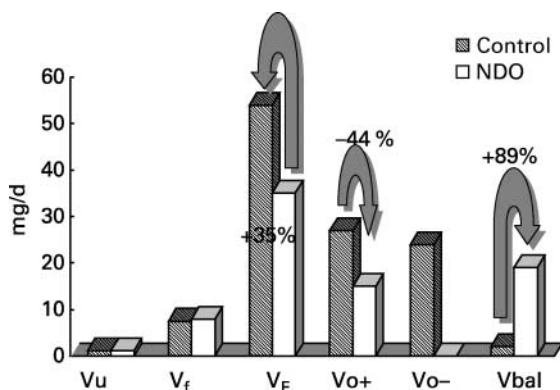
Fig. 2. Effect of feeding non-digestible oligosaccharides (NDO; inulin-enriched fructose) on rates of transport in rats. Values in mg/d: Vu, urinary calcium; Vf, endogenous calcium; VF, faecal calcium; VO+, bone formation rates; VO-, bone resorption rates; and Vbal, calcium balance. (From Zafar et al. (2004a,b).
