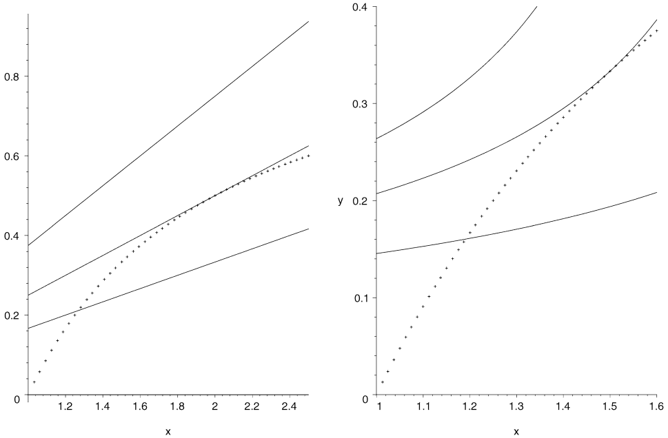
FIG. 1. Example 1.5.1: drawing f_{\mathbf{q}} for \alpha = 1/18, 1/12, 1/8 and x \mapsto 1 - 1/x (dashed) in the case \kappa = 2 of quadrangulations. Example 1.5.2: drawing f_{\mathbf{q}} for \beta = 1/7, 1/8, 1/10 and x \mapsto 1 - 1/x (dashed).
