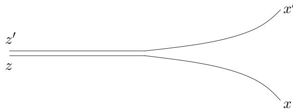
Figure 3: The distance function \kappa(x, x') might be constant for small \tau and increase exponentially later.
