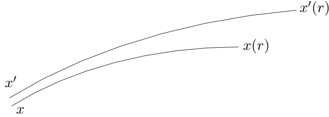
Figure 2: Ratner’s H-property: When moving along the unipotent u(r) , the points x(r) and x'(r) noticeably differ first only along U_{(12)} .
