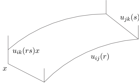
Figure 1: One key ingredient of the proof of Lemma 3.3 in [3] is the translation produced along U_{ik} when going along U_{ij} and U_{jk} and returning to the same leaf U_{ik}x .
