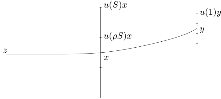
Figure 4: From the way the leaf U_{12}x is contracted along \alpha^{-t} we can ensure (4.13) if y = \alpha^{-wt}x \in \mathcal{X}_\rho
