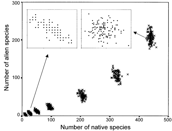
FIG. 4. Relationship between the number of alien species and number of native species at equilibrium over a range of community sizes (NAR; 100 realizations of simulated data for each community size). Individual point clusters correspond to communities of different sizes (numbers of individuals) ranging from 20 to 2000; inset plots are based on (left) communities of 50 individuals and (right) 2000 individuals only. Disturbance = 0.5, local replacement rate = 0.5; pool of alien species = 10 000, pool of native species = 500. All species are identical, except immigration rates of native species are 100 times higher than those of alien species.
