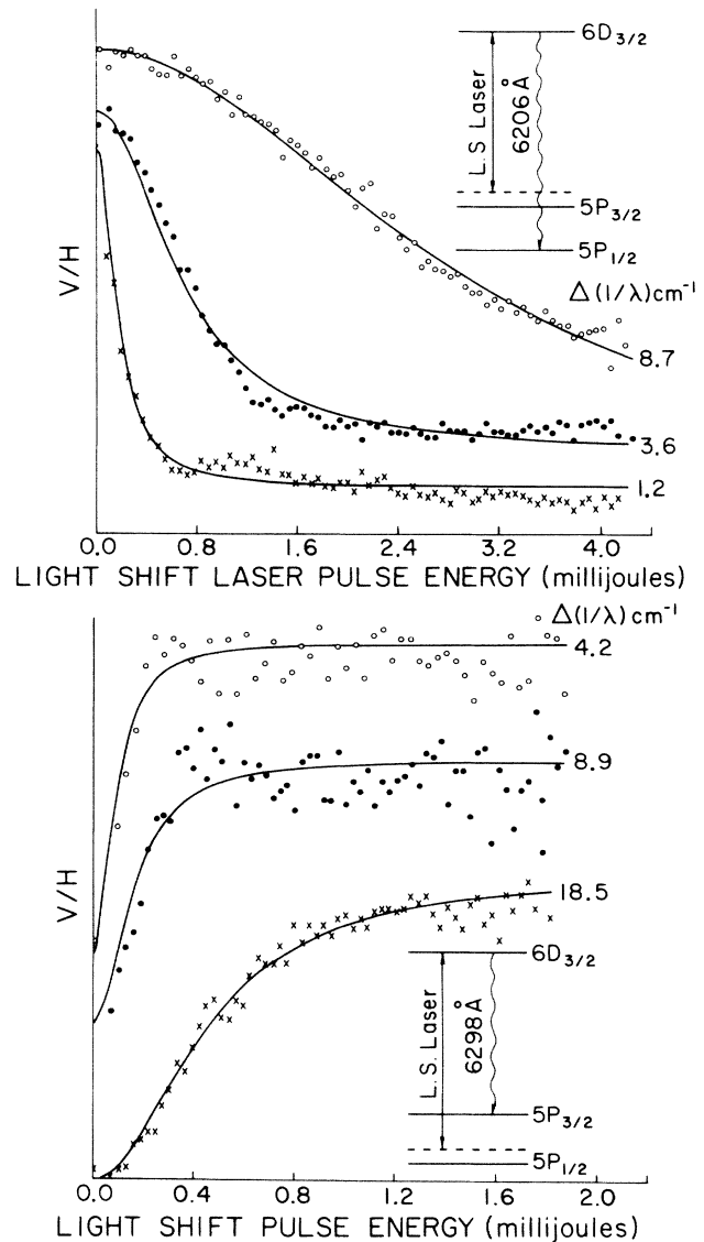
FIG. 3. Curves of the fluorescent polarization vs light-shift-pulse energy for various detunings \Delta(1/\lambda) . Light-shift laser wavelengths are indicated by solid lines, while detected fluorescence transitions are represented by wiggly lines.
