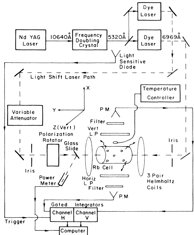
FIG. 2. Experimental apparatus.
