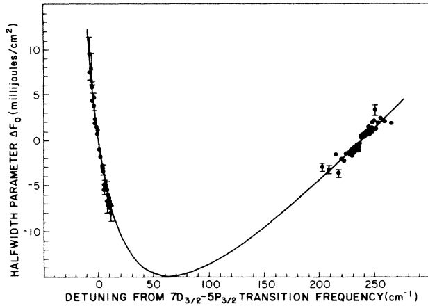
FIG. 4. Comparison of theory (solid line) from (9) with experimental data. We have set |\Delta F_0| equal to the widths of curves similar to those in Fig. 3 obtained for the 7D_{3/2} - 5P_{3/2} transitions. The sign of \Delta F_0 was chosen to agree with that predicted by (8).
