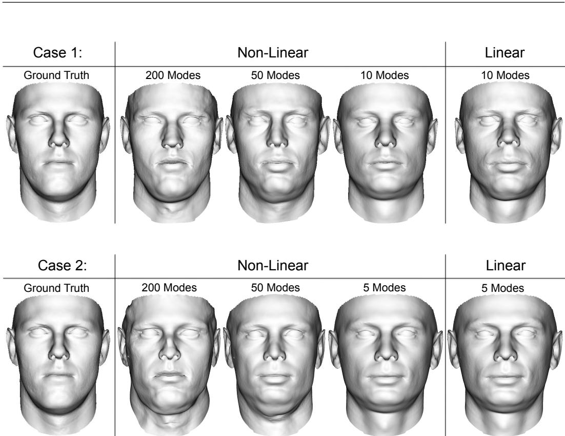
Figure A.6: Generalisation Results. Ground truth projected into the corresponding models.
