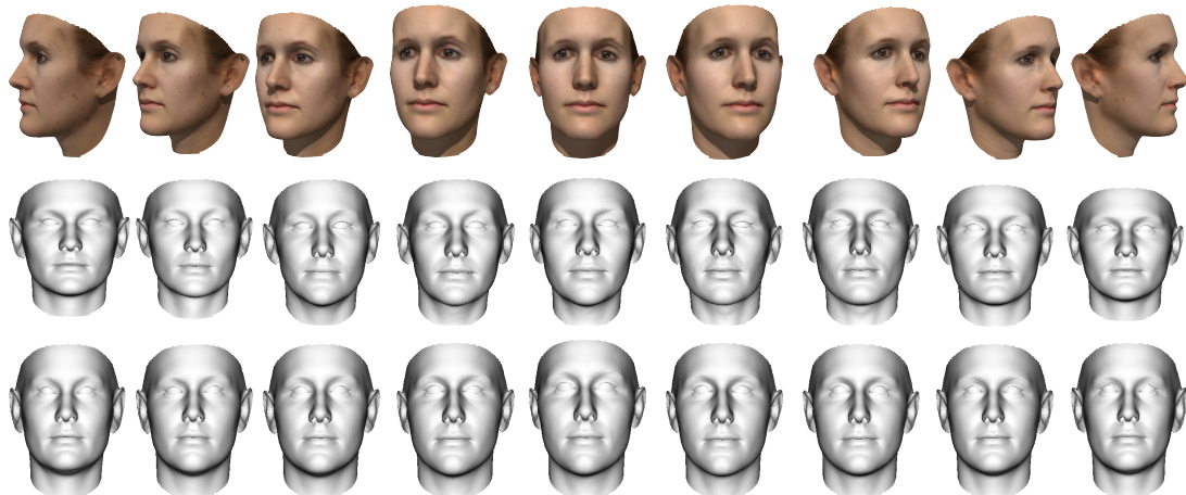
Figure 3.5: Fitting results for subject 323 in 9 pose angles. Top row shows renderings. Second row shows fitting results for the comparison method. Last row shows fitting results for the proposed method.
