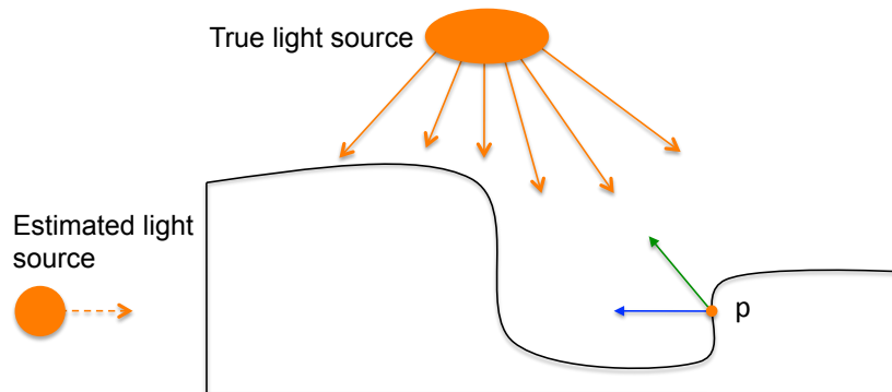
Figure 5.3: SH basis functions constructed from surface normals (blue arrow) would associate a non-existing light source to the reflectance at point p . Bent normals (green arrow) provide a better approximation of the true underlying illumination for non-convex objects.
