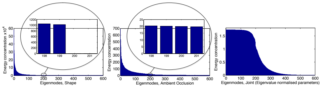
Figure 5.13: Eigenvalue decay for the three models. The magnification around the 200 th eigenvalue suggests a non-linear relationship between shape and ambient occlusion.
