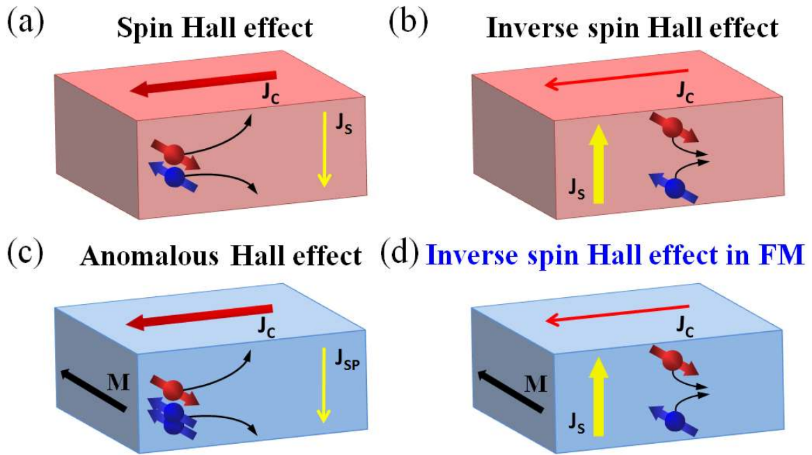
Fig. 1 (color online). Schematic diagrams of (a) spin Hall effect, (b) inverse spin Hall effect in a non-magnetic metal as well as (c) anomalous Hall effect, (d) inverse spin Hall effect in a ferromagnetic metal, illustrating the generation of charge current ( J_c ), spin current ( J_s ) and spin-polarized current ( J_{SP} ) from the transport of spin-up and spin-down electrons.
