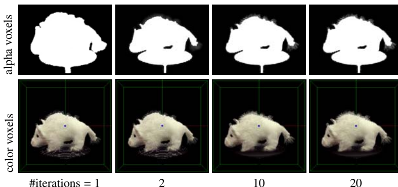
Fig. 6. Iterative optimization
