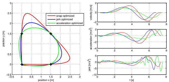
Fig. 7: Result of different optimization strategies for flying through the four points marked with “+”. Red denotes the resulting trajectory from optimizing over the snap, blue for jerk and green for acceleration. The right side shows the trajectories for the x-axis for velocity (top), acceleration (center) and jerk (bottom), again with the same color coding for the different methods.
