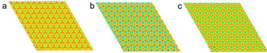
Supplementary Figure S9. Simulated STM images of different stacking orders. (a) AB-0. (b) AB-V4. (c) AB-V3. The bias voltage for imaging the valence band was chosen in the simulation. The images show that different configurations do not generate significant change in STM topology images, which is, most likely, because the states of top surface Se atoms dominate the appearance of topographic images. These results confirm the difficulty of distinguishing domains with different stacking orders in STM measurements. These IDB defects, showing strong metallic feature, significantly affect the contrast of STM images, making it difficult for one to pick up the minor variations (if any) of STM contrasts for different defect-free stacking domains..
