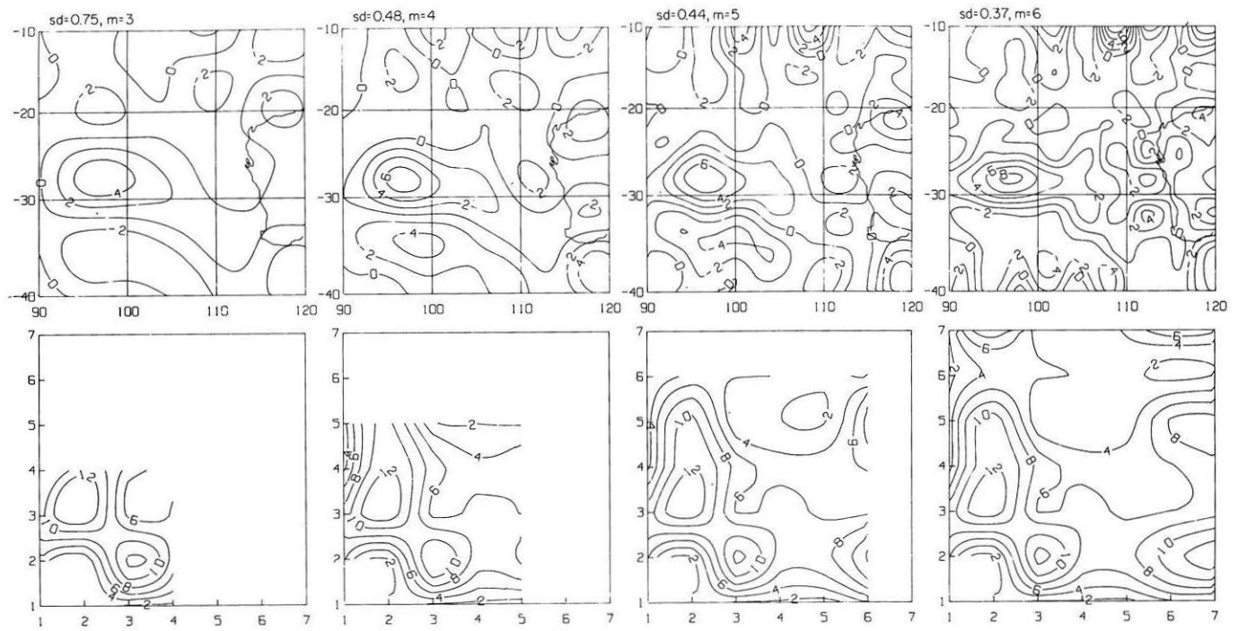
Fig. 8. Magnetization distributions and corresponding amplitude spectra for maximum wave number m=3, 4, 5, and 6 . Scale shown is wave number plus one. Units are 10^{-1} \text{Am}^{-1} . sd is the standard deviation of the fit between observed anomaly field and that computed from the magnetization distributions
