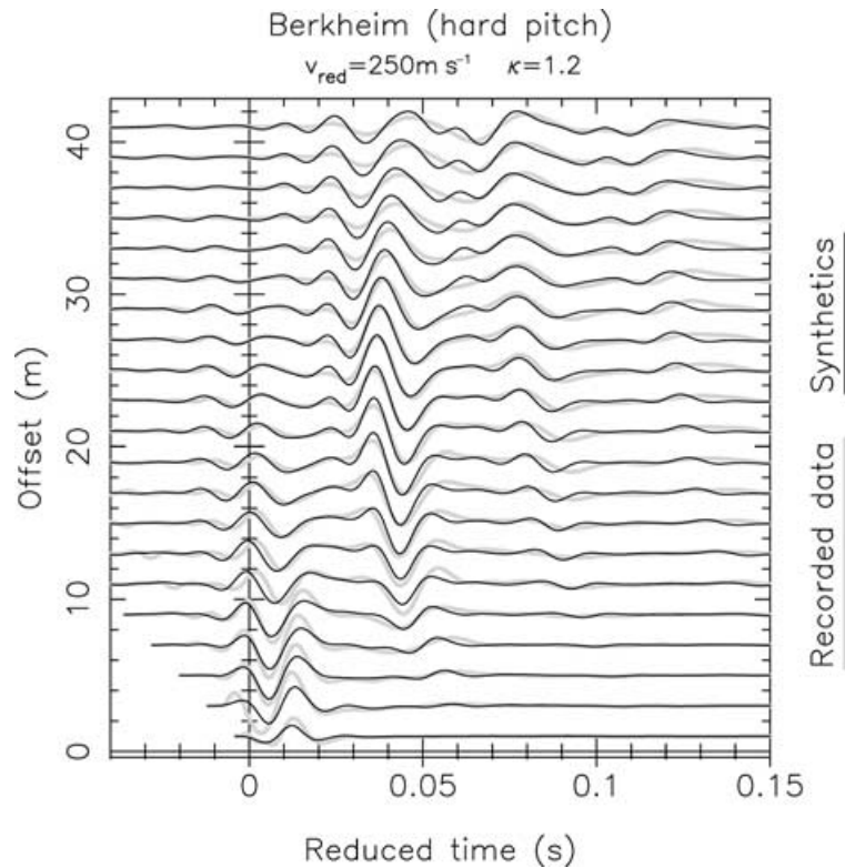
Figure 11. Data set Berkheim: Synthetic waveforms calculated from the final model (Fig. 8) are superimposed on the recorded seismograms (grey curves). The source wavelet (Fig. 12, top) derived from the (\omega, p) spectrum was used in the calculation. While the overall waveforms match very well, it is obvious that attenuation of high frequencies is still too weak in the synthetics.
