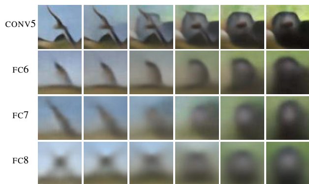
Figure 10: Interpolation between the features of two images.
