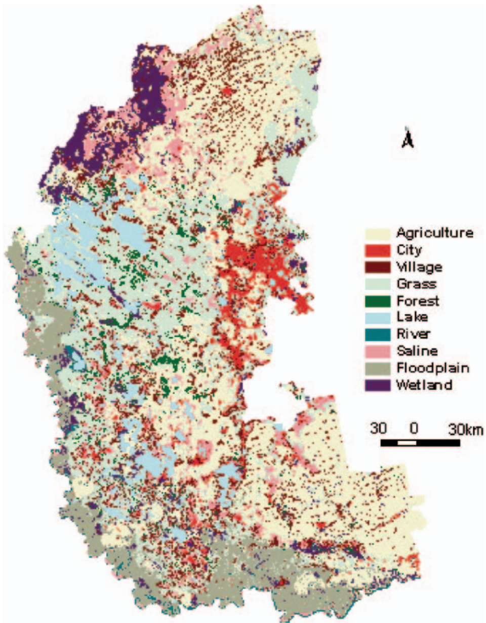
Figure 2. The landscape pattern map of Daqing city in 2000.
