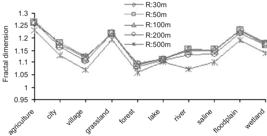
Figure 4. Comparison of fractal dimension of landscape classes at different scales.
