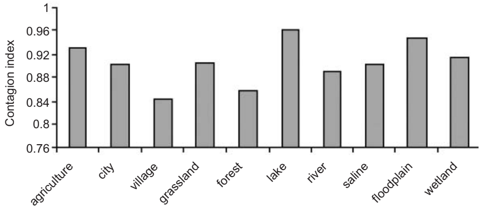
Figure 5. Contagion index for landscape classes.
