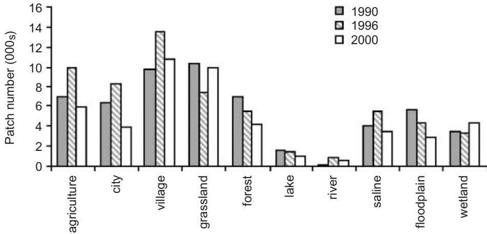
Figure 8. Comparison of landscape patch number of each class between 1990 and 2000.
