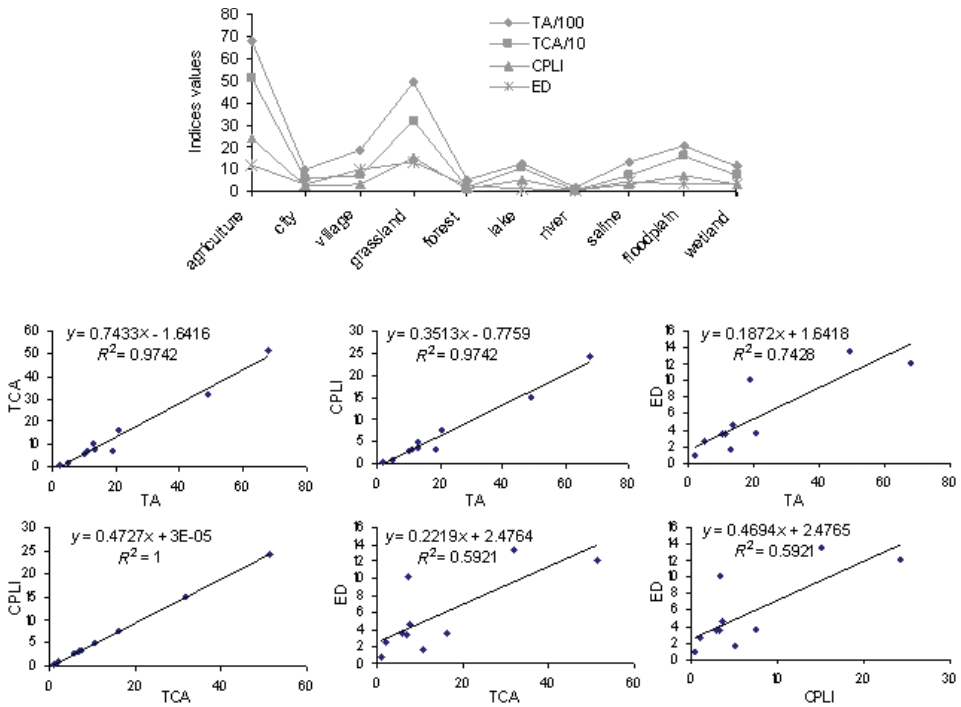
Figure 6. The relationship between total area, core area, core percentage landscape index, and edge density.
