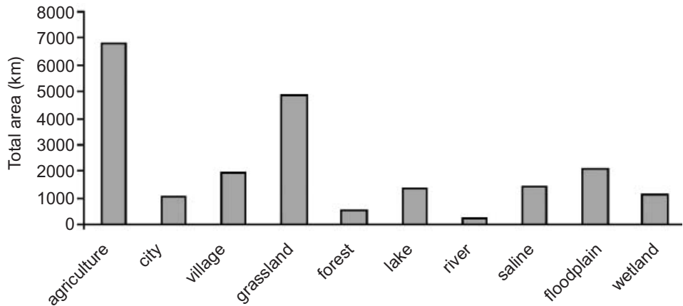
Figure 3. Area of landscape classes.
