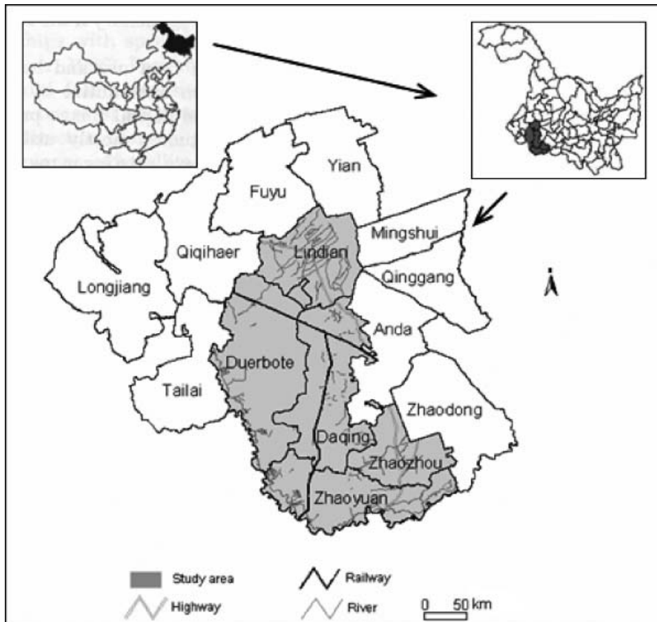
Figure 1. Study area, Daqing city, China.
