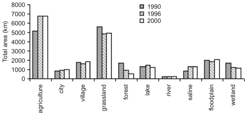
Figure 7. Comparison of landscape area of each class between 1990 and 2000.
