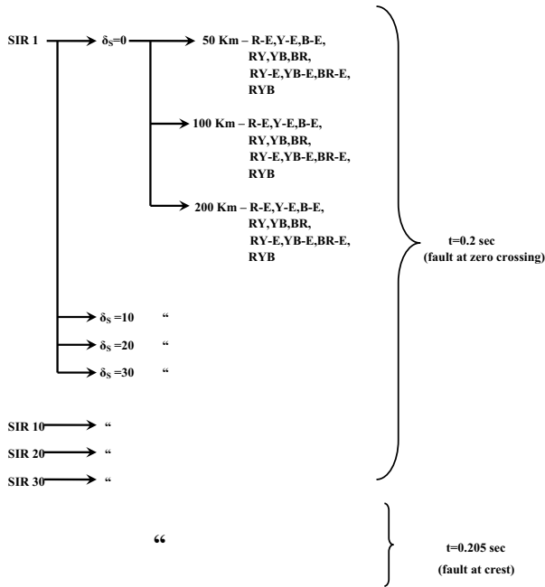
Fig. 7: Simulation cases carried out to investigate numerical distance relay performance
