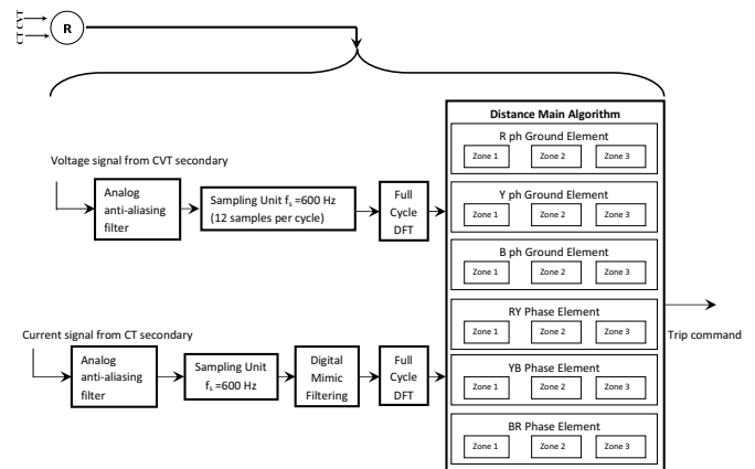
Fig. 6: Developed numerical distance relay model in SIMULINK
