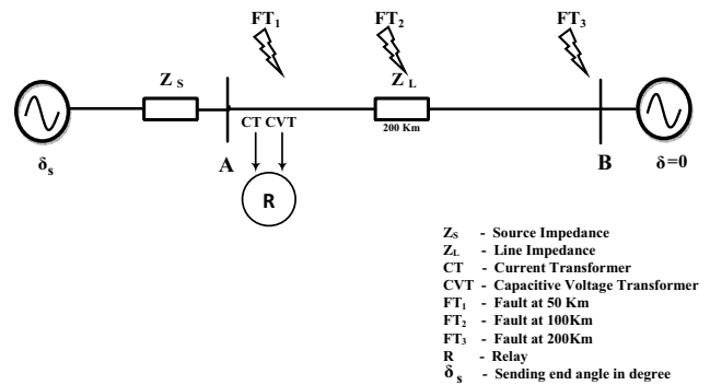
Fig. 5: Single line diagram of 400KV test system
