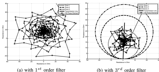
Fig. 11: Impedance loci with 1^{st} and 3^{rd} order filter for YB phase fault at t = 0.2 sec and at 100 km ( SIR = 30 , \delta_s = 0 )
