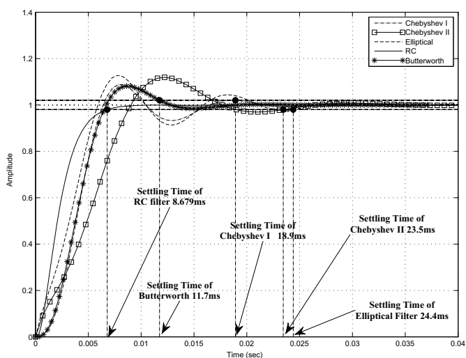
Fig. 1: Step Response of analog antialiasing filters
