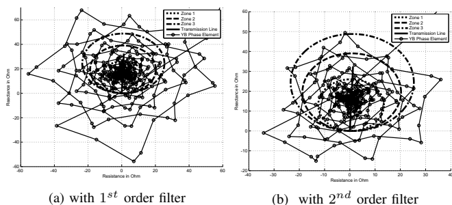
Fig. 10: Impedance loci with 1^{st} and 2^{nd} order filter for YB phase fault at t = 0.2 sec and at 100 km ( SIR = 30 , \delta_s = 30 )
