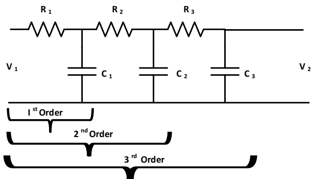
Fig. 2: Model of RC filter
