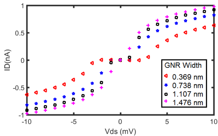
Figure 3: SET current versus drain voltage for different island widths, gate voltage is 1mV and GNR length is 0.492 nm.
