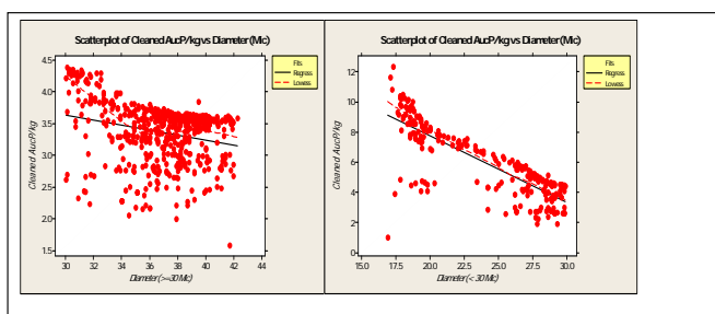
Figure 2. Scatter plots developed from simple linear regression model for diameter ( \geq 30 micron) and diameter (< 30 micron) from left to right.
