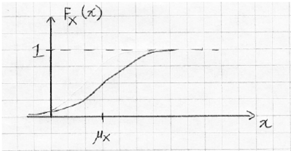
Fig. 4 Distribution function F(x) X .
