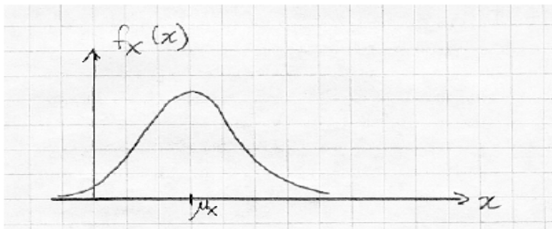
Fig. 5 Density function f(x) X .
