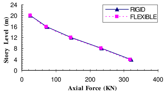
FIG.9- Axial forces of C4 in Rectangular building without shear walls under X-X direction earthquake
