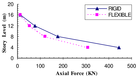
FIG 6-Axial forces of C2 in L-shaped building without shear walls under Y-Y direction earthquake
