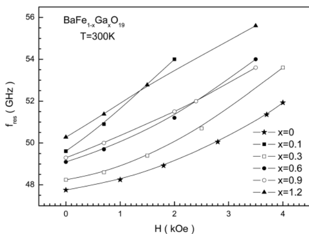
Fig. 11 The external magnetic bias field dependence of the f_{res}(H) NFR frequency at T = 300 K for BaFe_{12-x}Ga_xO_{19} ( x = 0; 0.1; 0.3; 0.6; 0.9; \text{ and } 1.2 ) solid solutions.
