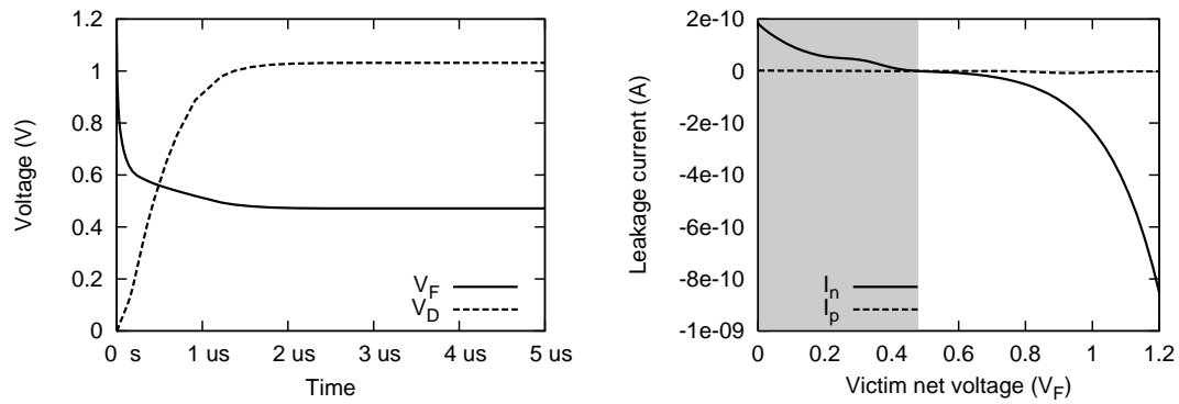
(a) The victim net voltage V_F and the drain voltage V_D (b) The leakage current through the NMOS and PMOS transistors I_N , I_P
