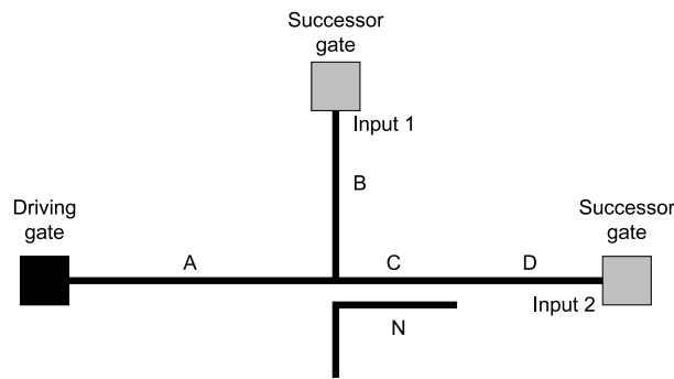
FIGURE 4.3: Net segmentation representing possible defect locations
