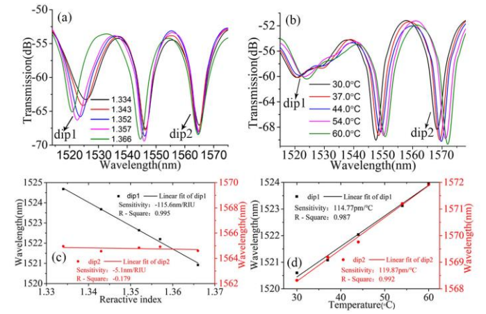
Fig. 7. Transmission spectra of dip1 and dip2: (a) versus RI; (b) versus temperature. Linear fit diagram of dip1 and dip2 wavelength shift: (c) versus RI; (d) versus temperature.
