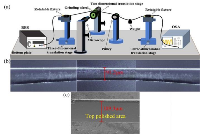
Fig. 3. (a) Fiber side polished system diagram. (b) The photo of side-polished fiber under microscope. (c) The SEM image of the top polished area.
