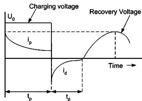
Fig. 2. Dielectric response measurement.
